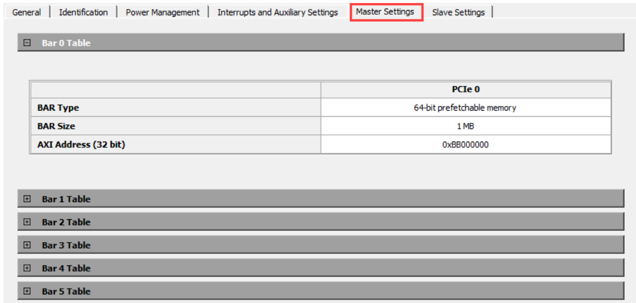
Figure 1-12. Example of Configuring Master RP Settings
