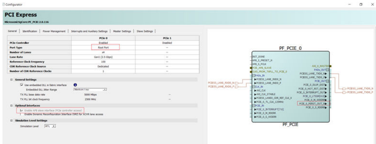
Figure 3-10. PCIe Configurator When PCIe is Configured as a PCIe Root Port
