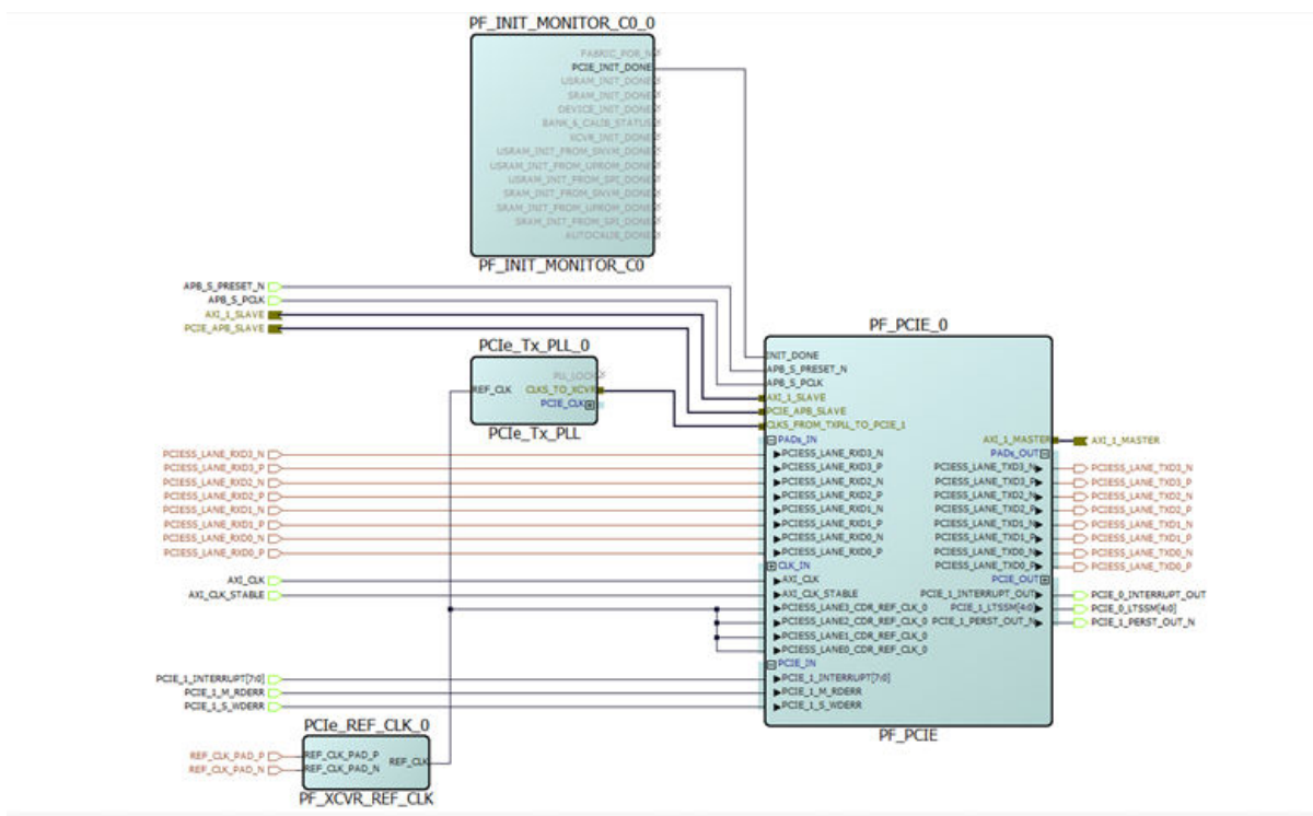
Figure 3-11. Complete PCIe Interface Example with PERSTn Signal
