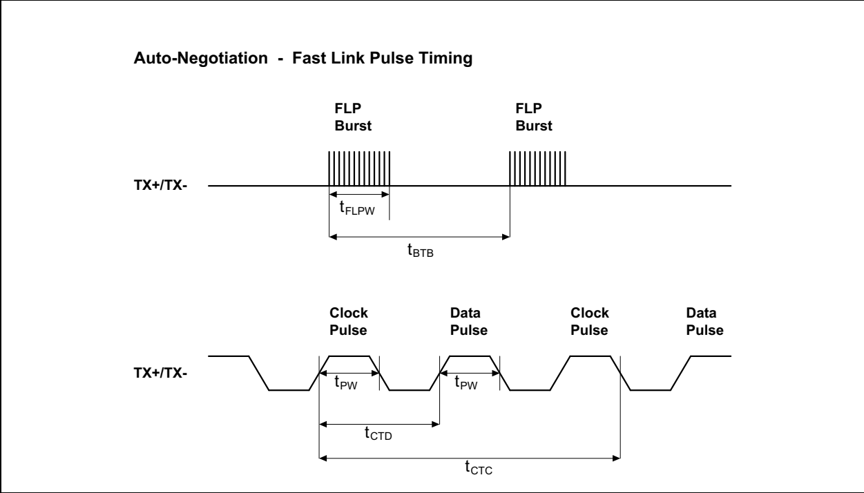
FIGURE 7-13: AUTO-NEGOTIATION TIMING
