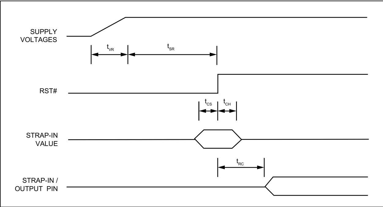
FIGURE 7-15: RESET TIMING
