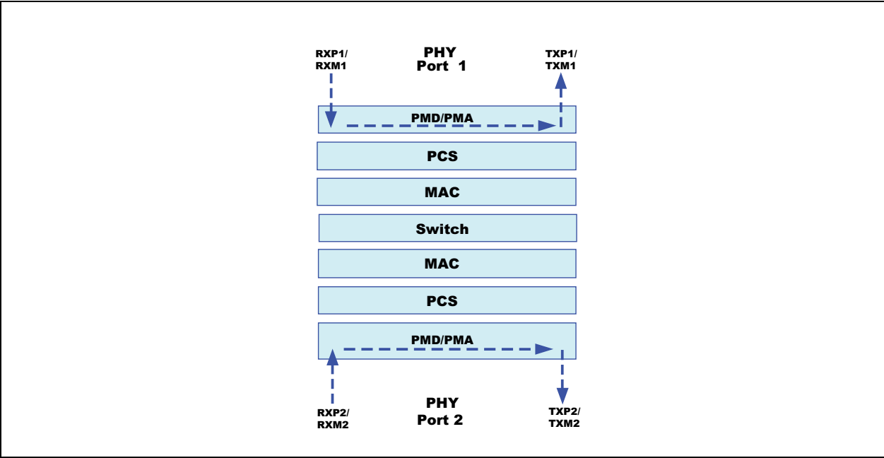
FIGURE 3-13: NEAR-END (REMOTE) LOOPBACK PATH
