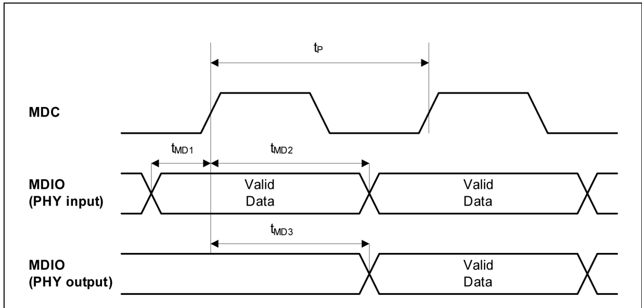
FIGURE 7-14: MDC/MDIO TIMING
