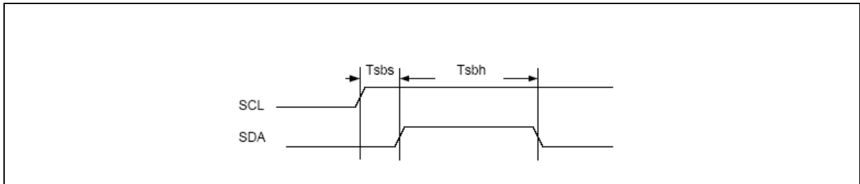
FIGURE 7-9: I 2 C STOP BIT TIMING
