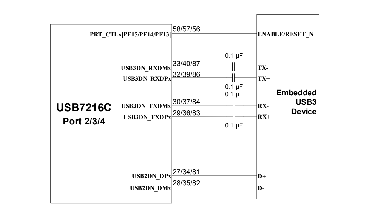
FIGURE 4-10: DOWNSTREAM PORTS 2, 3, OR 4 EMBEDDED DEVICE USB CONNECTIONS
