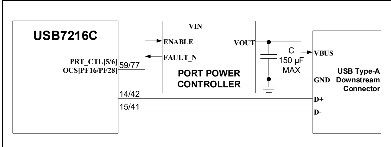
FIGURE 4-11: DOWNSTREAM PORTS 5 AND 6 VBUS AND PRT_CTLX CONNECTIONS
