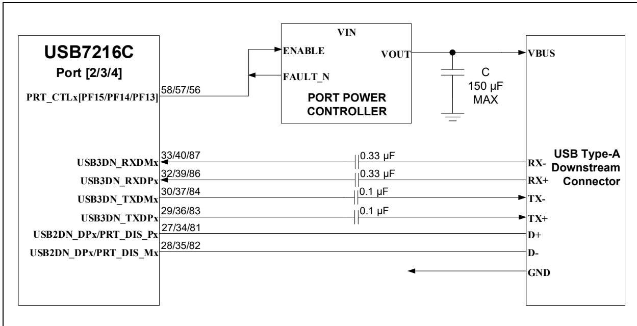
FIGURE 4-9: DOWNSTREAM PORTS 2, 3, AND 4 USB SIGNAL AND VBUS CONNECTIONS
