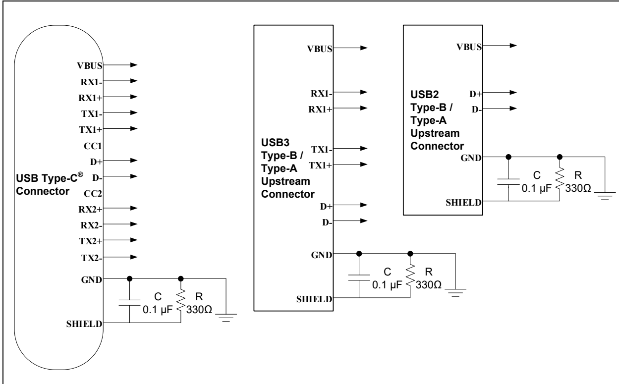
FIGURE 4-12: RECOMMENDED USB CONNECTOR GND AND SHIELD CONNECTIONS
