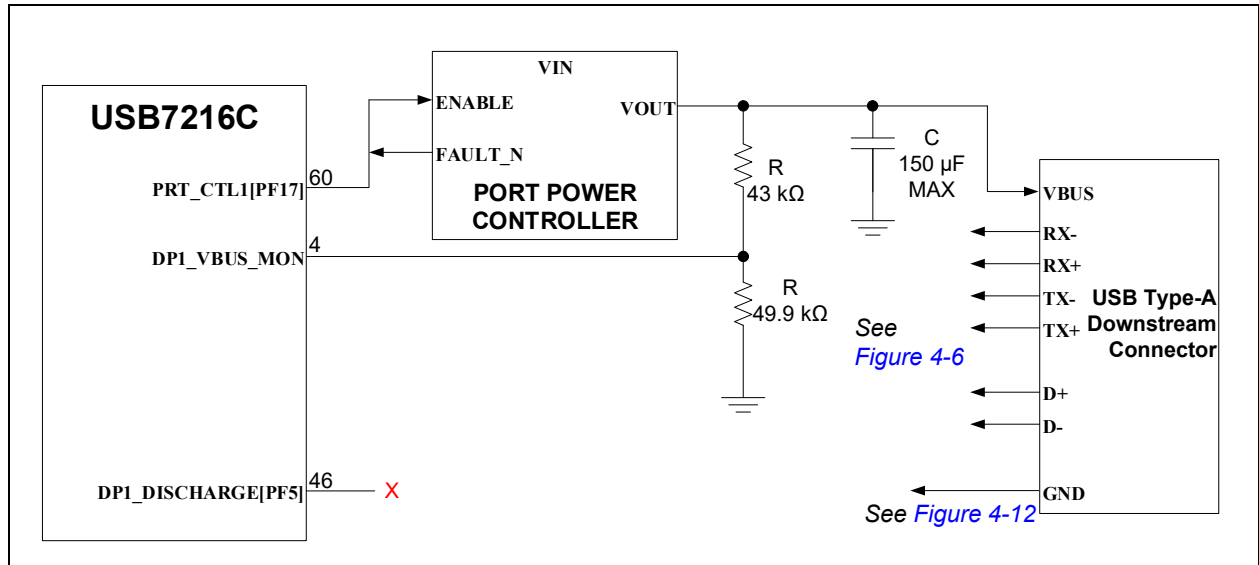
FIGURE 4-7: DOWNSTREAM PORT 1 VBUS AND PRT_CTLX CONNECTIONS FOR TYPE-A PORT
