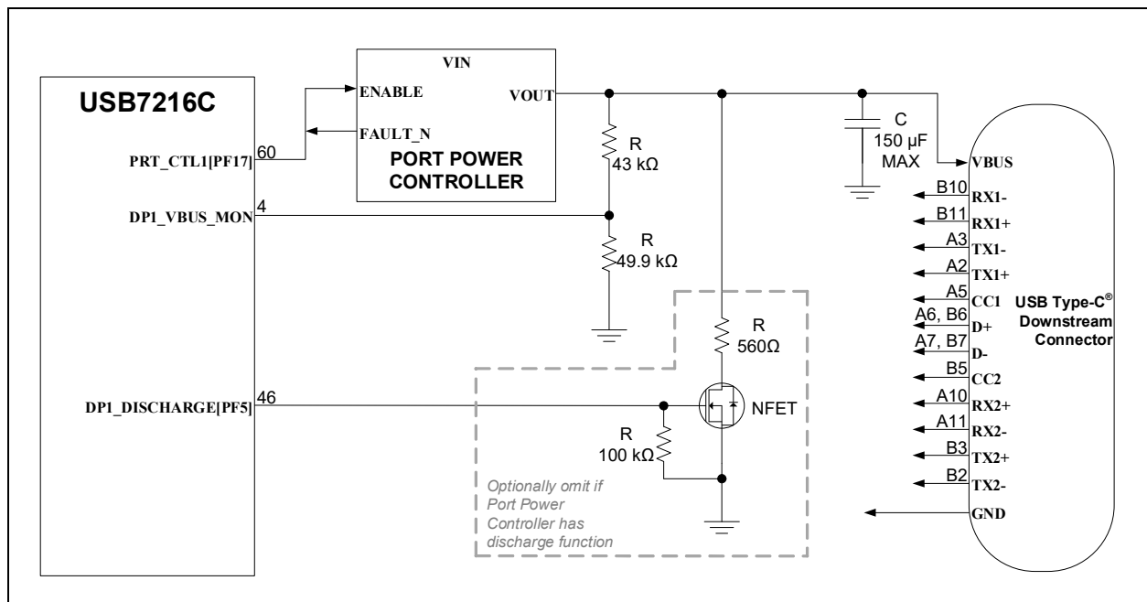
FIGURE 4-5: DOWNSTREAM PORT 1 USB TYPE-C® VBUS AND PRT_CTL CONNECTIONS
