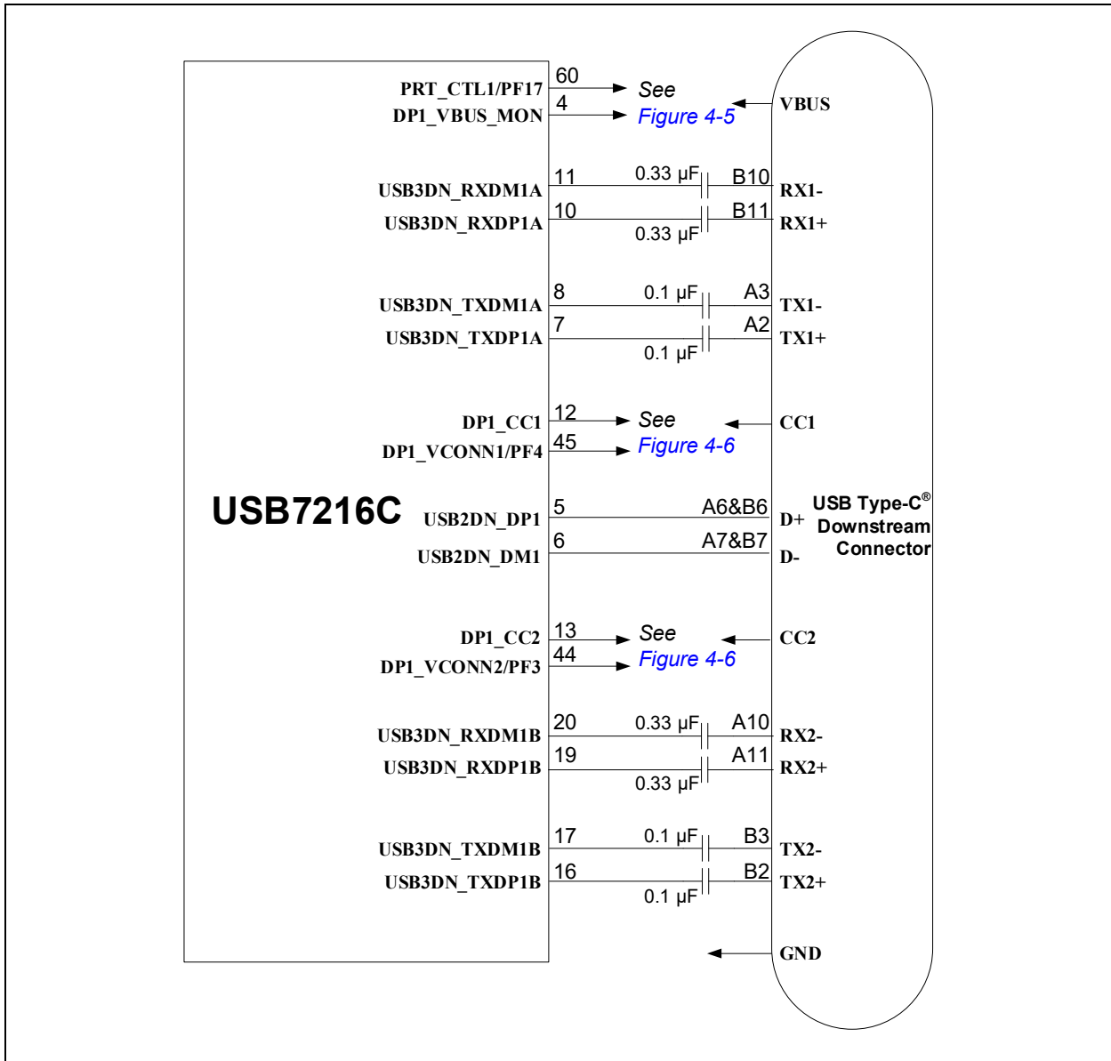
FIGURE 4-4: DOWNSTREAM PORT 1 TYPE-C® USB CONNECTIONS
