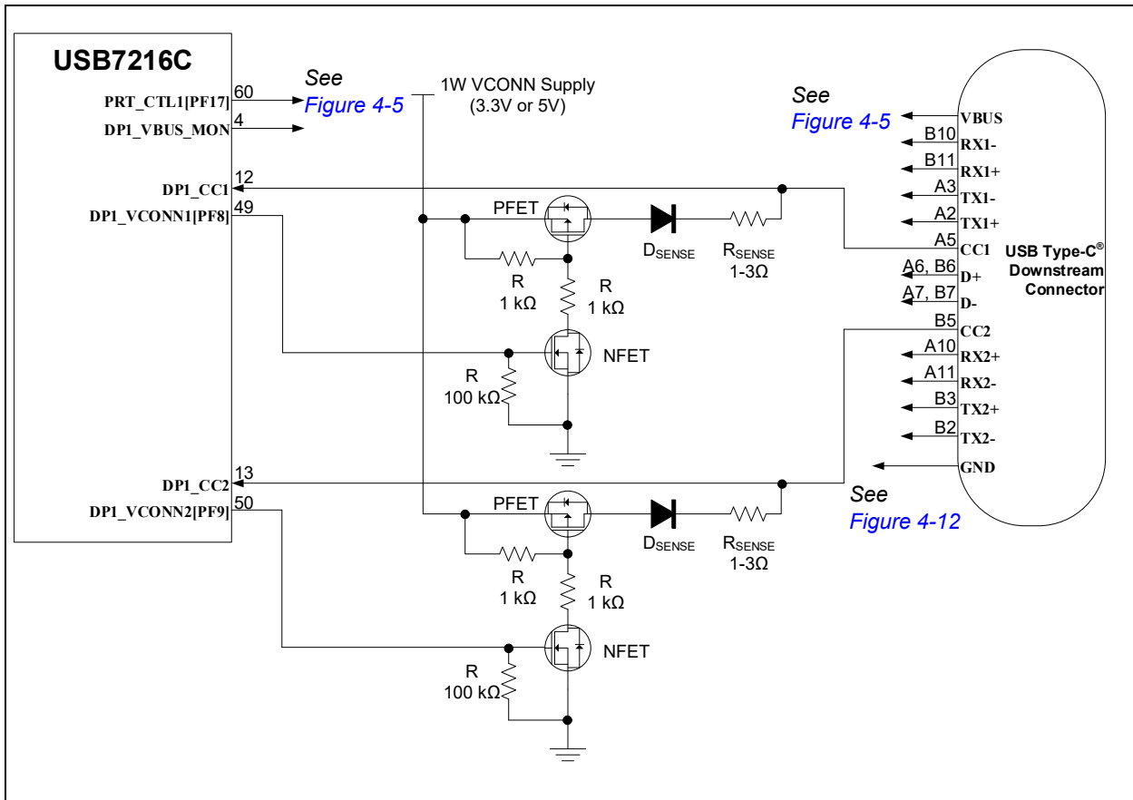
FIGURE 4-6: DOWNSTREAM PORT 1 CC1 AND CC2 CONNECTIONS
