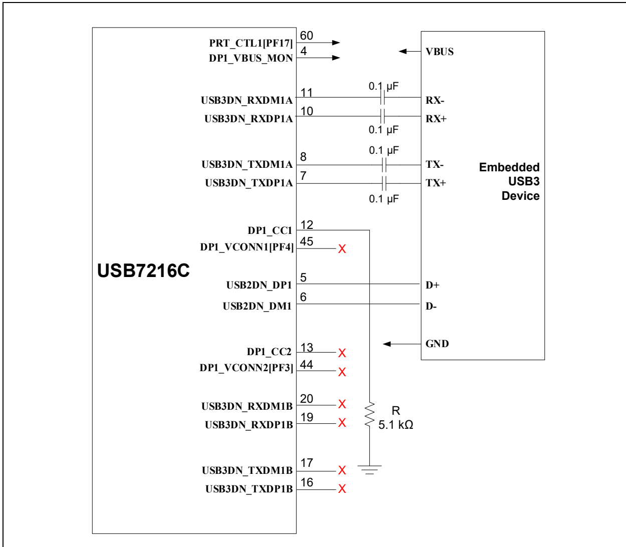
FIGURE 4-8: DOWNSTREAM PORT 1 EMBEDDED DEVICE USB CONNECTIONS
