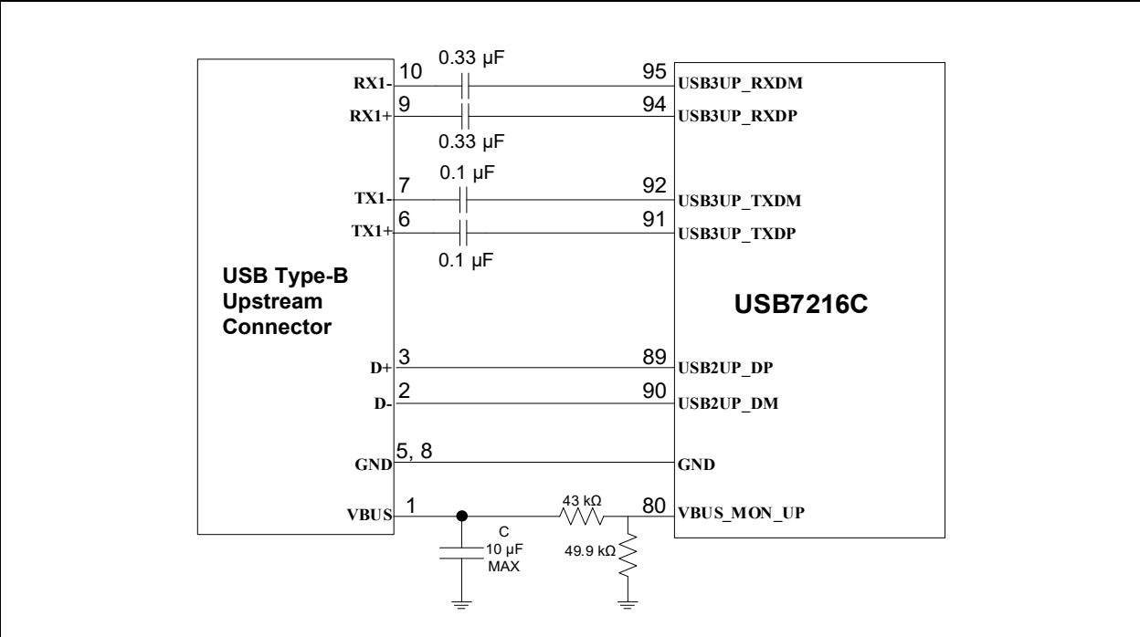
FIGURE 4-1: UPSTREAM PORT TYPE-B USB CONNECTIONS
