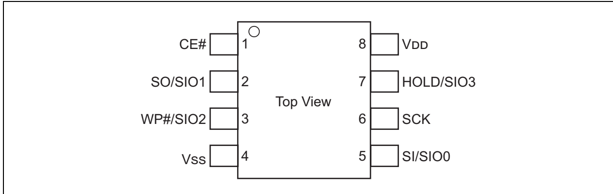
FIGURE 2-1: PIN DESCRIPTION FOR 8-LEAD SOIJ
