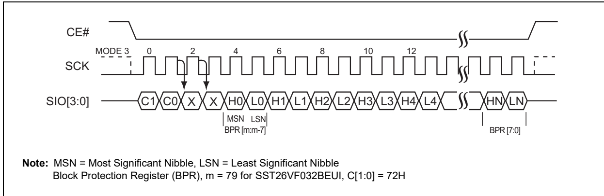
FIGURE 5-36: READ BLOCK PROTECTION REGISTER SEQUENCE (SQI)
