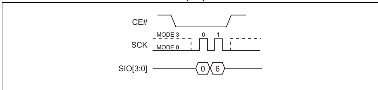
FIGURE 5-32: WRITE ENABLE SEQUENCE (SQI)
