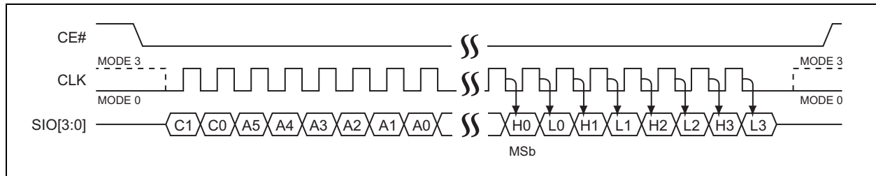
FIGURE 4-2: SQI SERIAL QUAD I/O PROTOCOL
