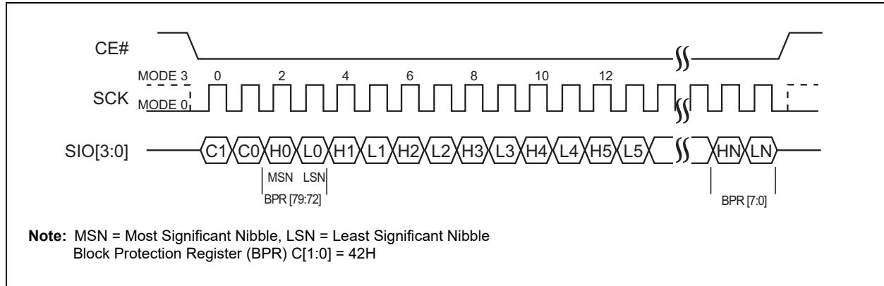
FIGURE 5-38: WRITE BLOCK PROTECTION REGISTER SEQUENCE (SQI)
