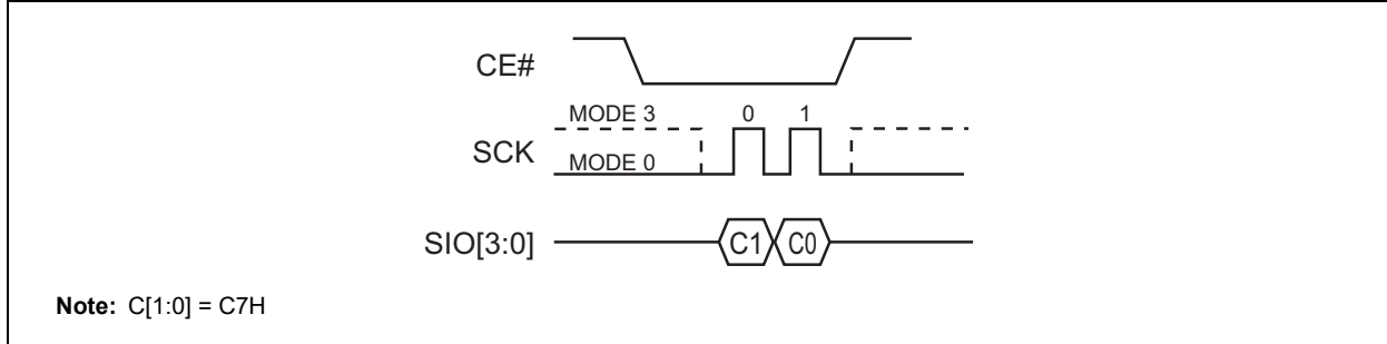
FIGURE 5-23: CHIP ERASE SEQUENCE (SQI)
