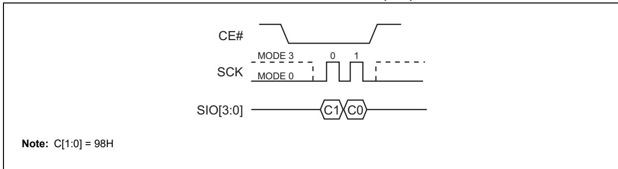
FIGURE 5-44: GLOBAL BLOCK PROTECTION UNLOCK (SQI)
