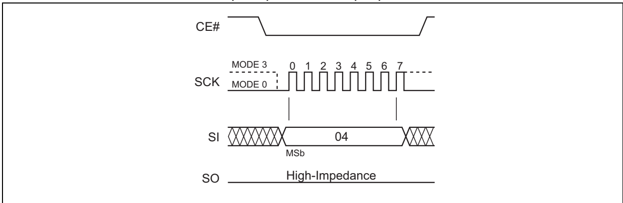
FIGURE 5-35: WRITE DISABLE ( WRDI ) SEQUENCE (SPI)
