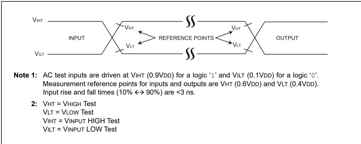
FIGURE 8-5: AC INPUT/OUTPUT REFERENCE WAVEFORMS
