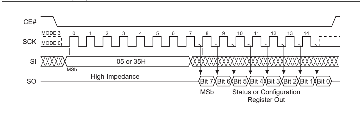
FIGURE 5-29: READ STATUS REGISTER AND READ CONFIGURATION REGISTER SEQUENCE (SPI)
