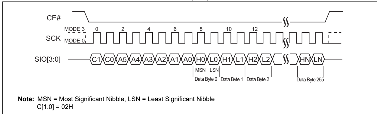
FIGURE 5-25: PAGE PROGRAM SEQUENCE (SQI)
