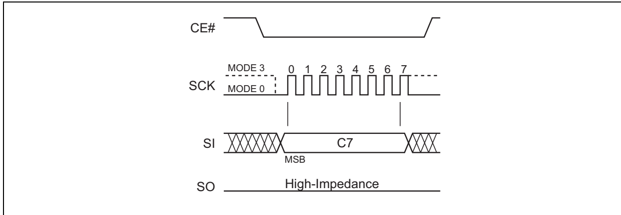
FIGURE 5-24: CHIP ERASE SEQUENCE (SPI)
