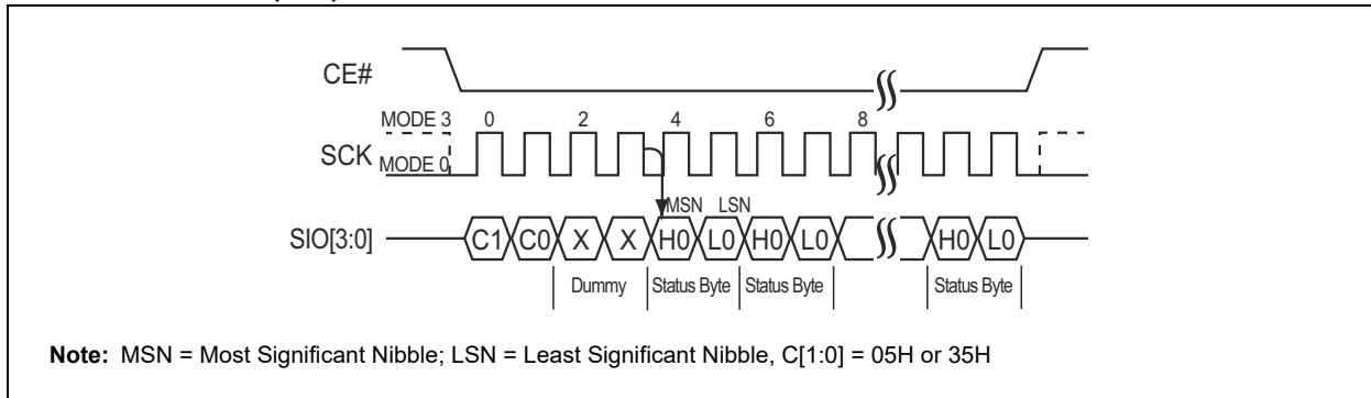
FIGURE 5-28: READ STATUS REGISTER AND READ CONFIGURATION REGISTER SEQUENCE (SQI)
