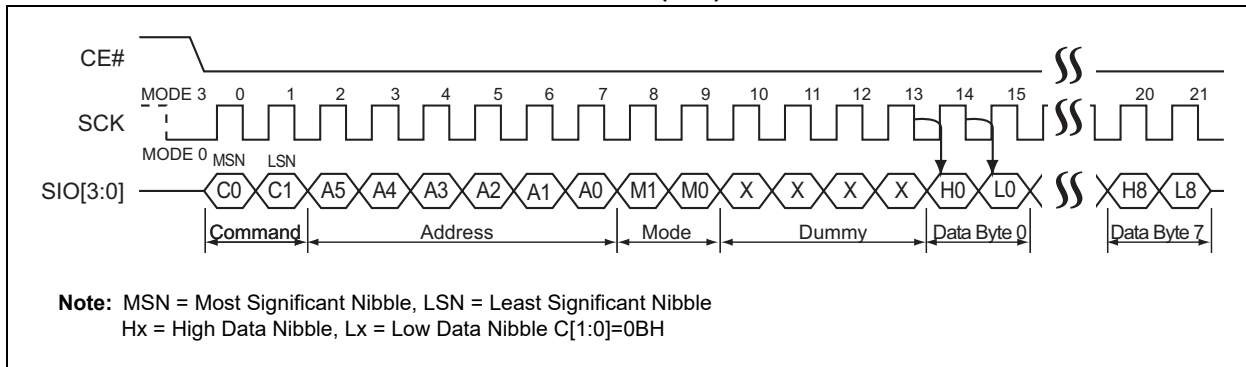
FIGURE 5-7: HIGH-SPEED READ SEQUENCE (SQI)
