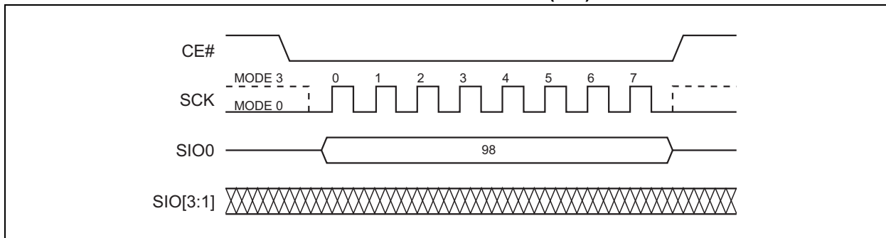
FIGURE 5-45: GLOBAL BLOCK PROTECTION UNLOCK (SPI)
