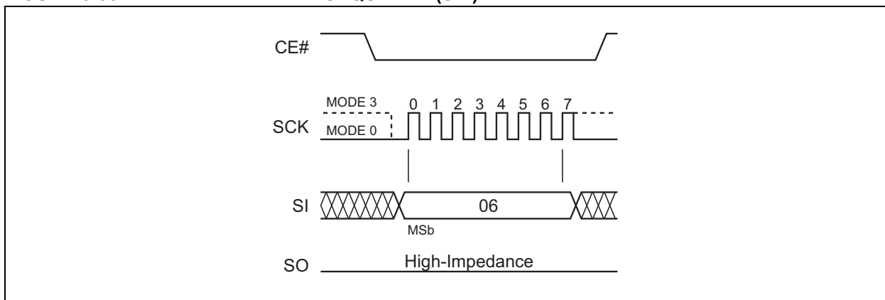
FIGURE 5-33: WRITE ENABLE SEQUENCE (SPI)
