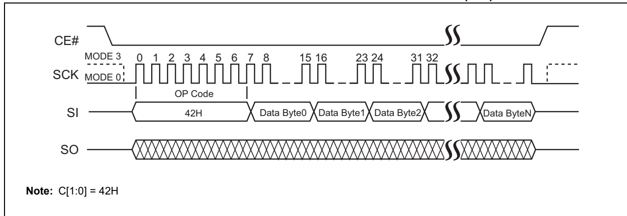
FIGURE 5-39: WRITE BLOCK PROTECTION REGISTER SEQUENCE (SPI)
