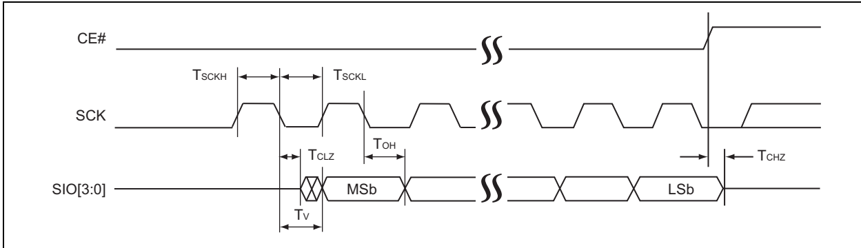
FIGURE 8-3: SERIAL OUTPUT TIMING DIAGRAM
