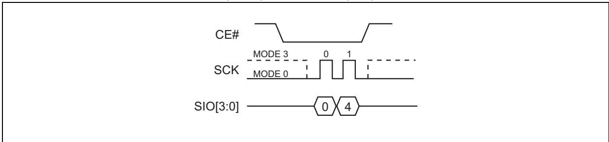
FIGURE 5-34: WRITE DISABLE ( WRDI ) SEQUENCE (SQI)
