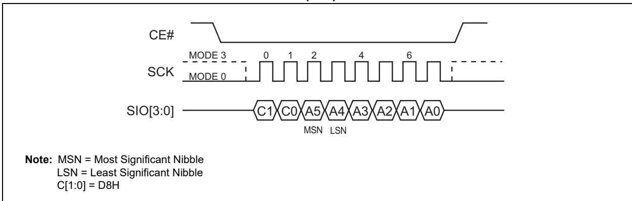
FIGURE 5-21: BLOCK ERASE SEQUENCE (SQI)
