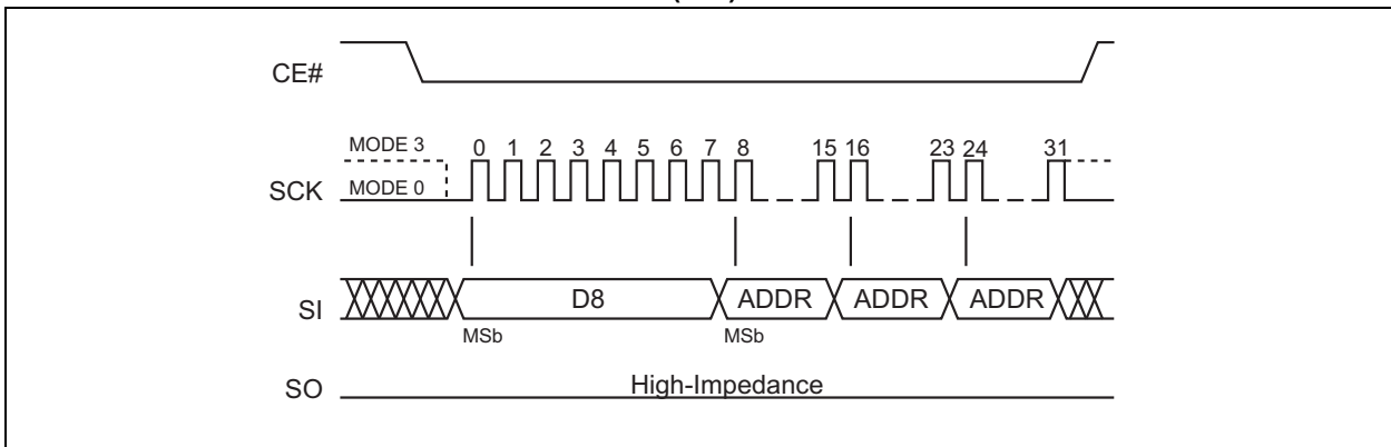
FIGURE 5-22: BLOCK ERASE SEQUENCE (SPI)
