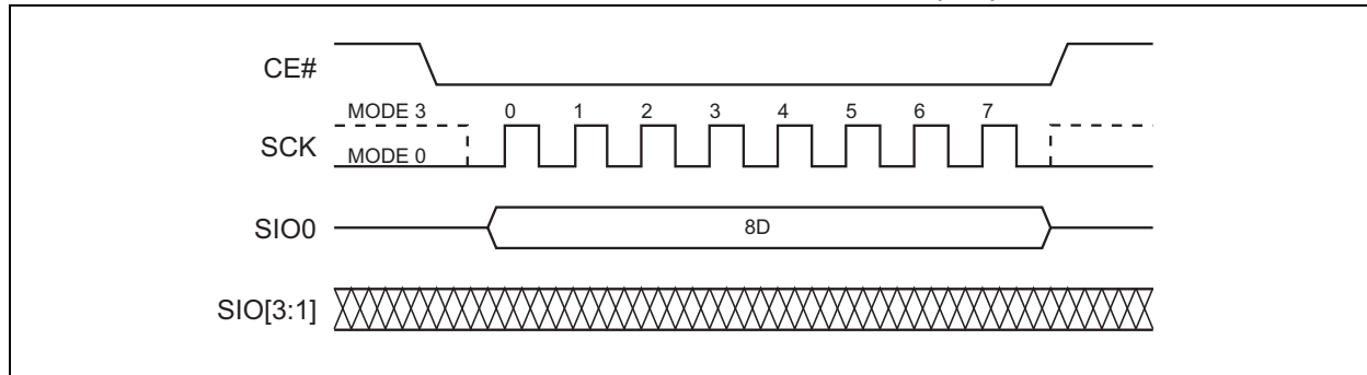
FIGURE 5-41: LOCK-DOWN BLOCK PROTECTION REGISTER (SPI)
