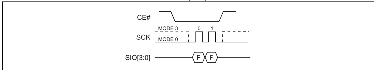
FIGURE 5-5: RESET QUAD I/O SEQUENCE (SQI)
