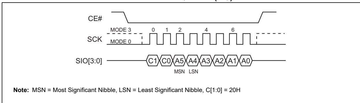
FIGURE 5-19: 4-KBYTE SECTOR ERASE SEQUENCE (SQI)
