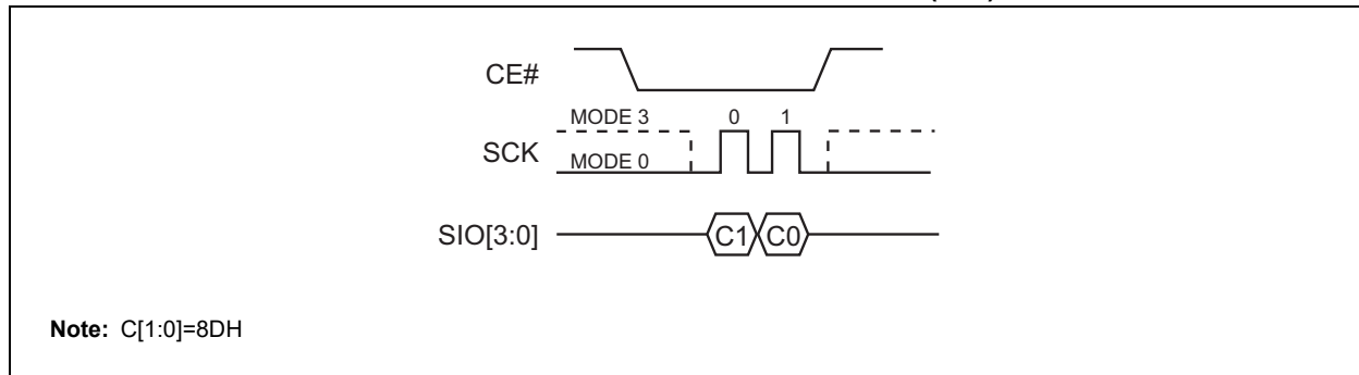
FIGURE 5-40: LOCK-DOWN BLOCK PROTECTION REGISTER (SQI)
