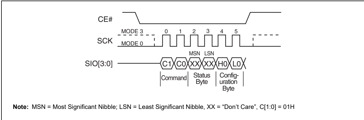
FIGURE 5-30: WRITE STATUS REGISTER SEQUENCE (SQI)
