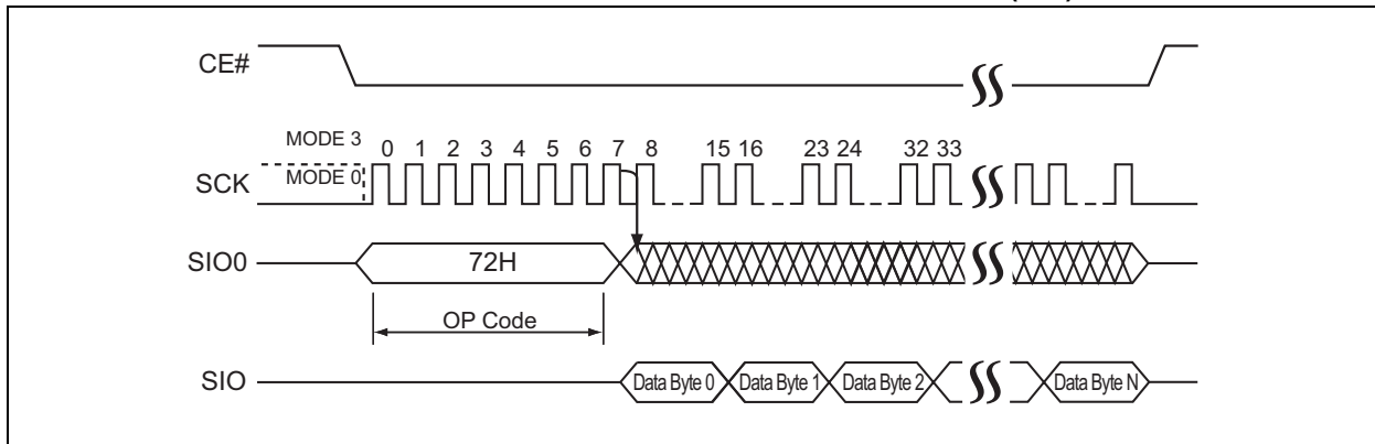
FIGURE 5-37: READ BLOCK PROTECTION REGISTER SEQUENCE (SPI)
