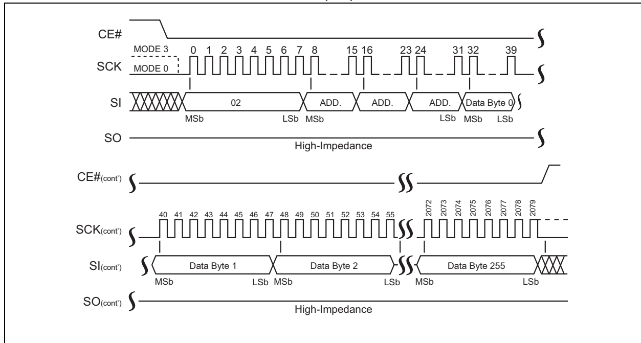
FIGURE 5-26: PAGE PROGRAM SEQUENCE (SPI)
