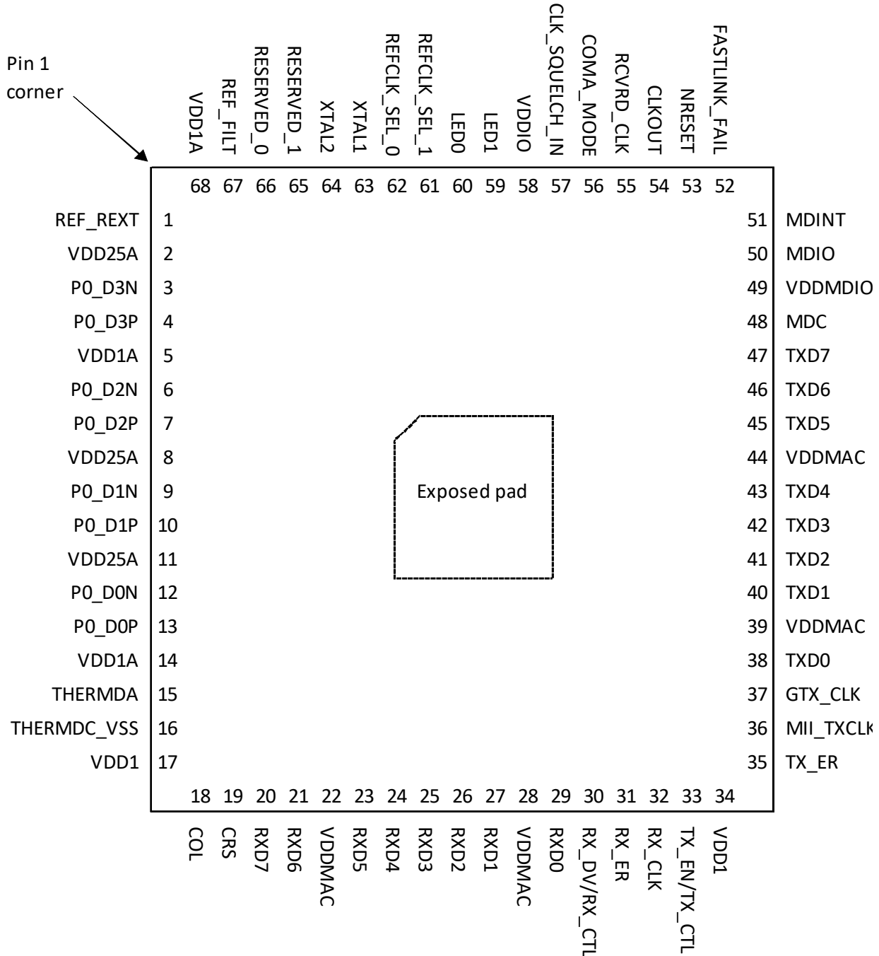
Figure 35 • Pin Diagram
