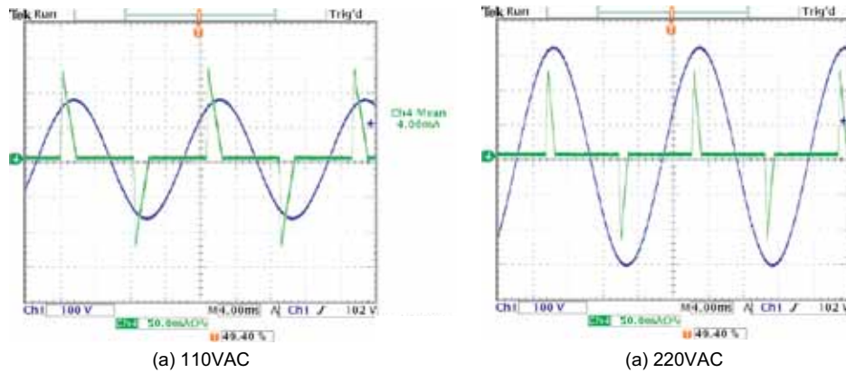
Fig.7 Input Voltage and Input Current Waveforms
