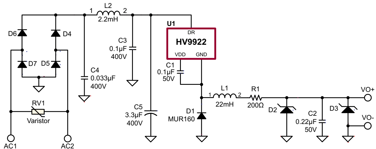
Circuit Schematic:
