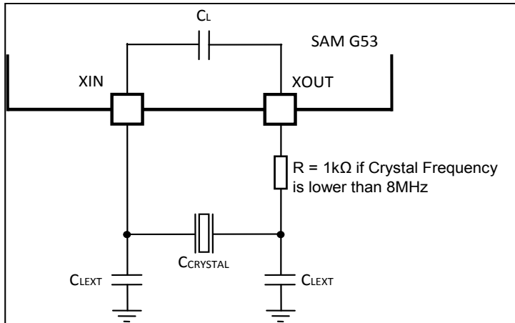
Figure 1-2. Main Crystal Schematic Example
