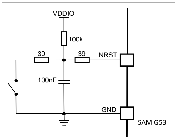
Figure 1-8. Reset Hardware Implementation
