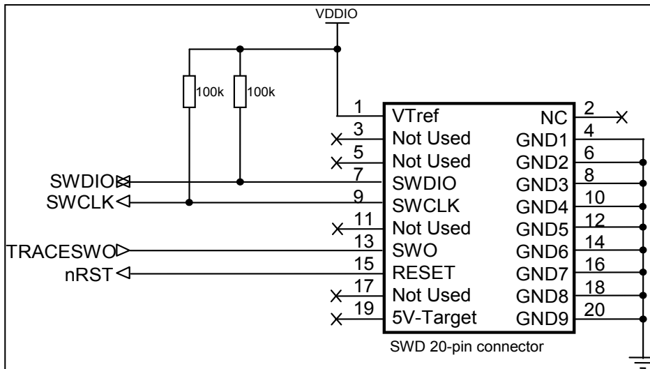
Figure 1-7. SWD Schematic Example: SWD 20-pin Connector
