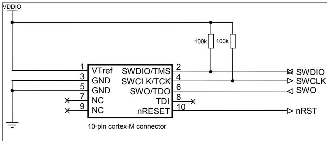
Figure 1-6. SWD Schematic Example: 10-pin Cortex-M Connector
