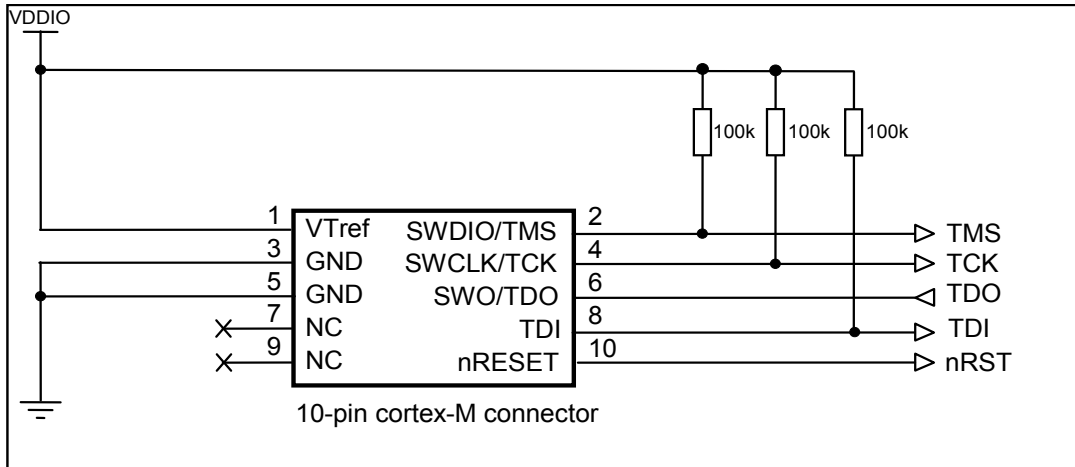
Figure 1-4. JTAG Schematic Example: 10-pin Cortex-M Connector
