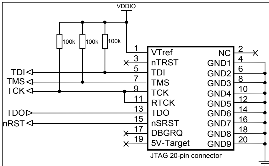
Figure 1-5. JTAG Schematic Example: JTAG 20-pin Connector
