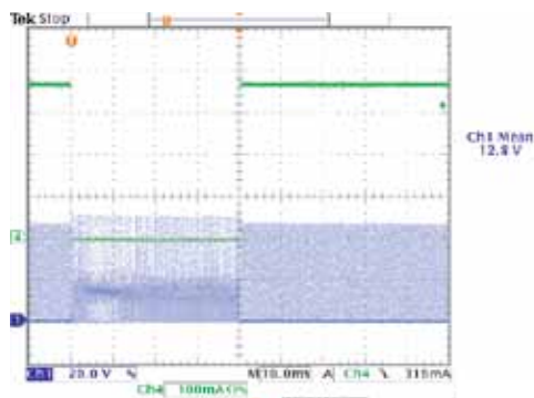
(a): Open LED Condition
