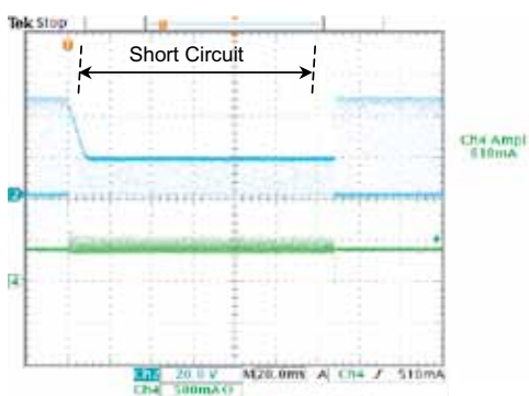
(b): Output Short Circuit
