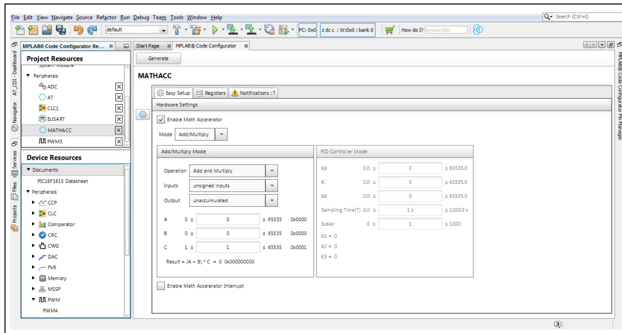
FIGURE F-3: MATH ACCELERATOR IN MCC FOR PIC16F1615
