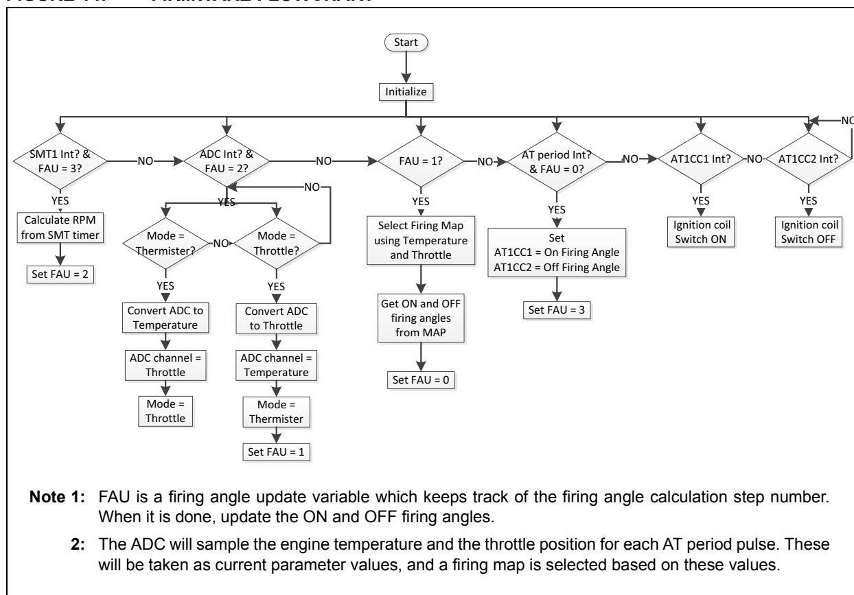
FIGURE 14: FIRMWARE FLOWCHART
