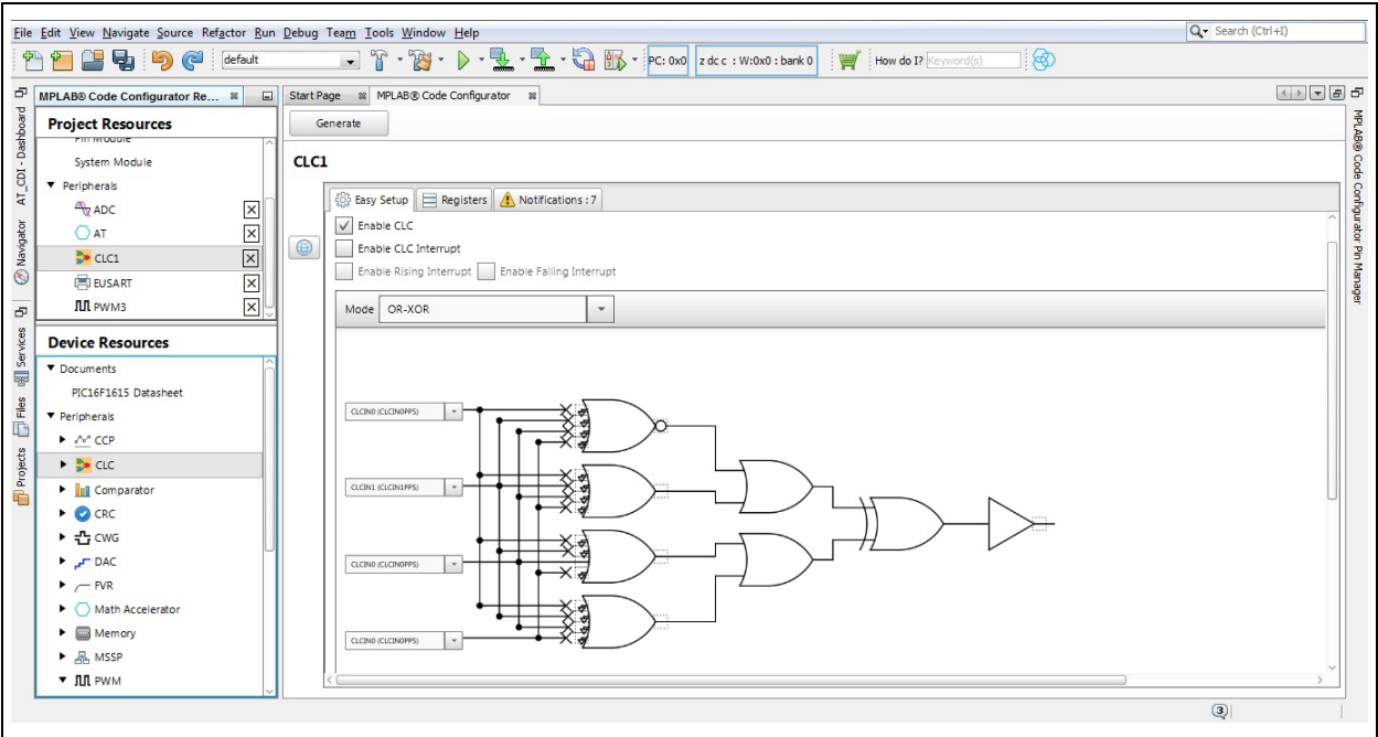
FIGURE F-2: CLC CONFIGURATION IN MCC FOR PIC16F1615
