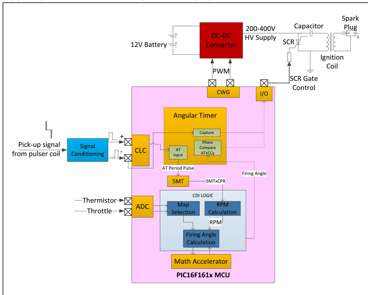
FIGURE 10: CDI IMPLEMENTATION WITH PIC16F161X
