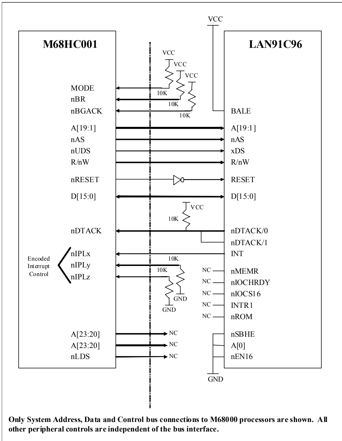
Figure 2.3 MC68HC001 (8-/16 BIT PROCESSOR)
