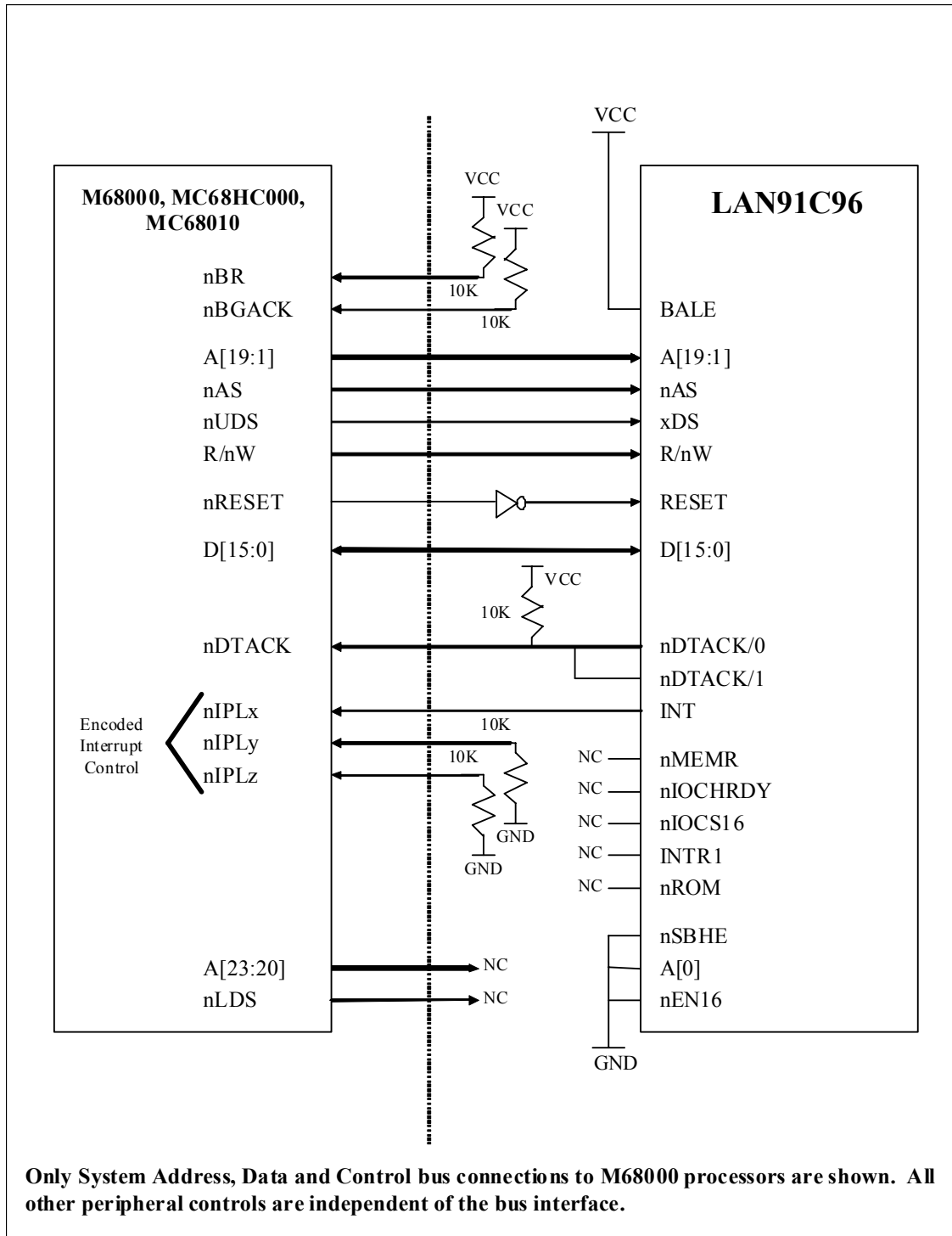
Figure 2.2 – MC68000, MC68HC000, AND MC68010 (16-BIT PROCESSORS)
