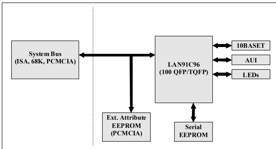
Figure 2.1 LAN91C96 SYSTEM BLOCK DIAGRAM
