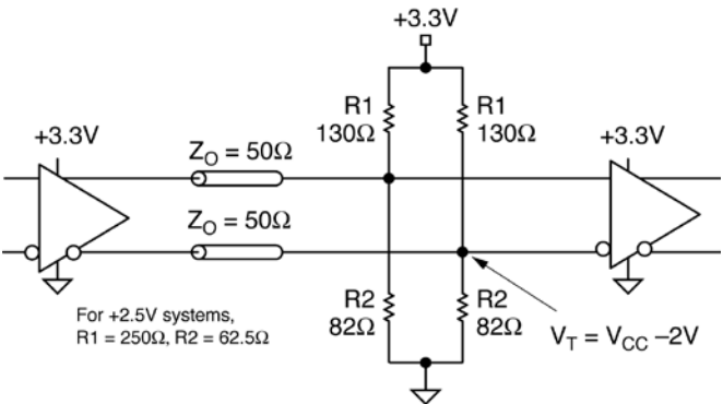
Figure 4a. Parallel Termination-Thevenin Equivalent
