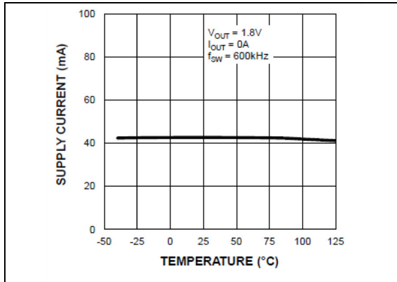
FIGURE 2-2: V_{IN} Operating Supply Current vs. Temperature (MIC45208-2).
