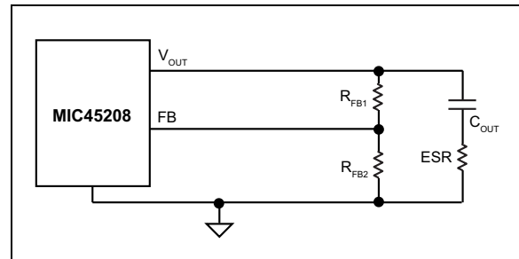
FIGURE 5-4: Enough Ripple at FB from ESR.
