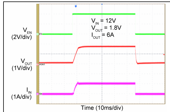
FIGURE 2-38: Inrush ( C_{OUT} = 3000\mu F ).
