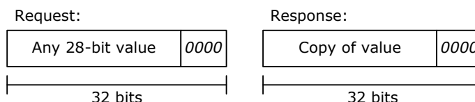
FIGURE 2-46: IDLE COMMAND
