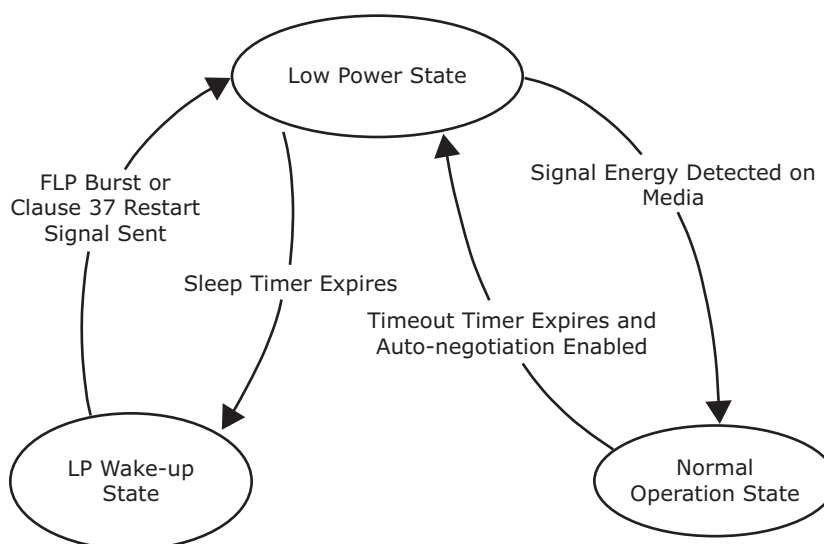
FIGURE 2-8: ACTIPHY STATE DIAGRAM
