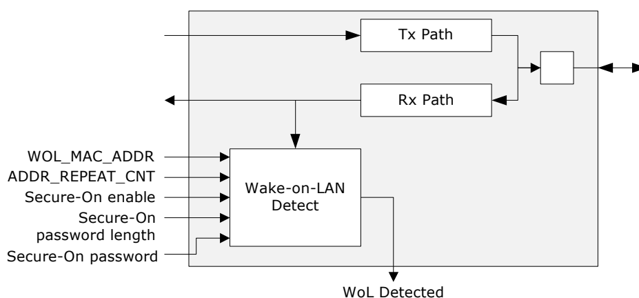
FIGURE 2-6: WAKE-ON-LAN FUNCTIONALITY
