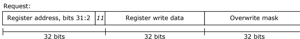
FIGURE 2-45: READ-MODIFY-WRITE COMMAND
