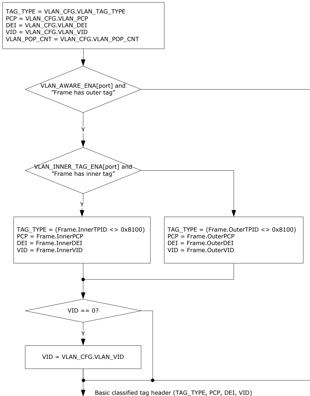
FIGURE 2-16: BASIC VLAN CLASSIFICATION FLOW
