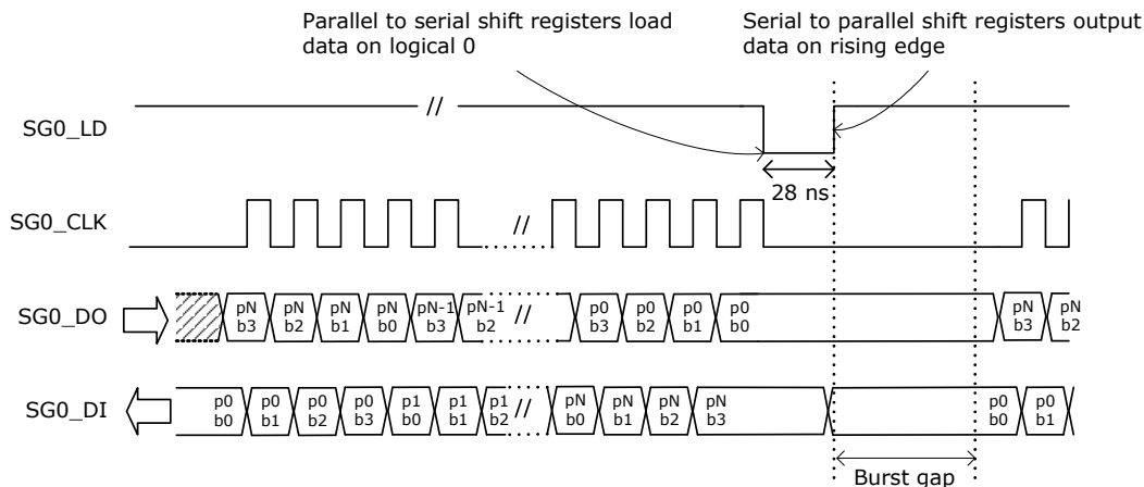
FIGURE 3-26: SIO TIMING
