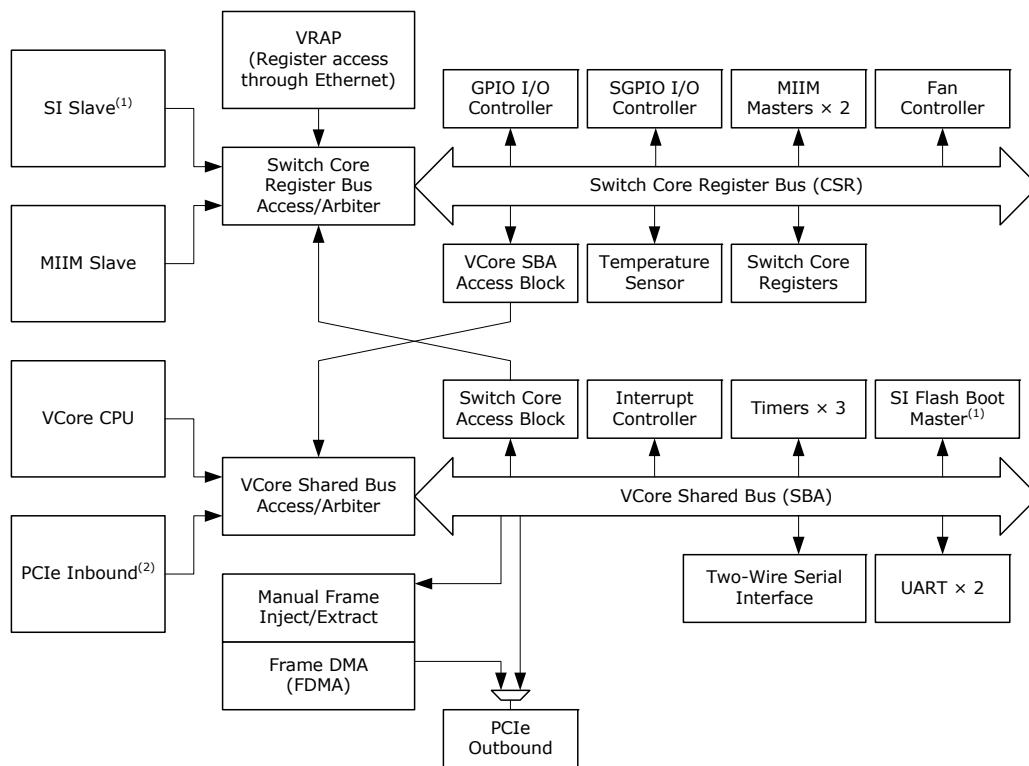
FIGURE 3-1: VCORE-IE SYSTEM BLOCK DIAGRAM
