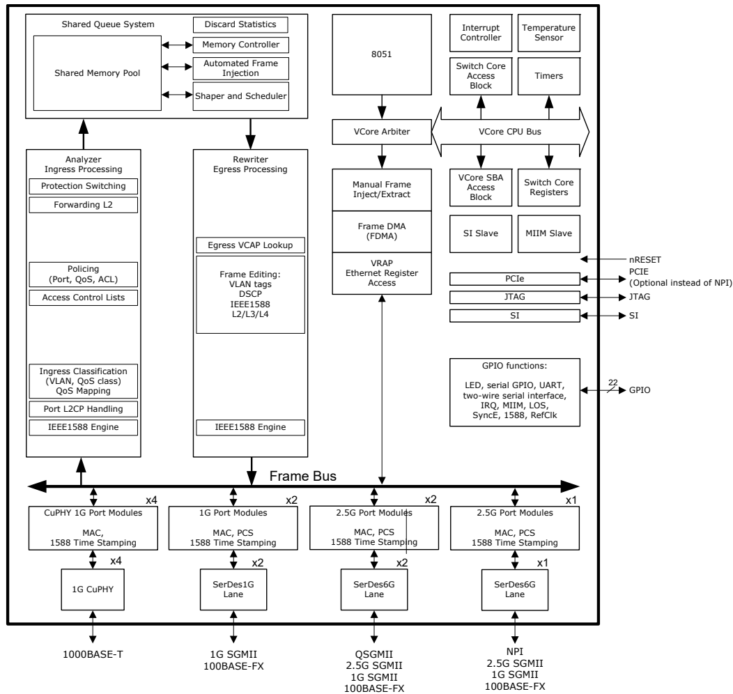
FIGURE 1-1: BLOCK DIAGRAM
