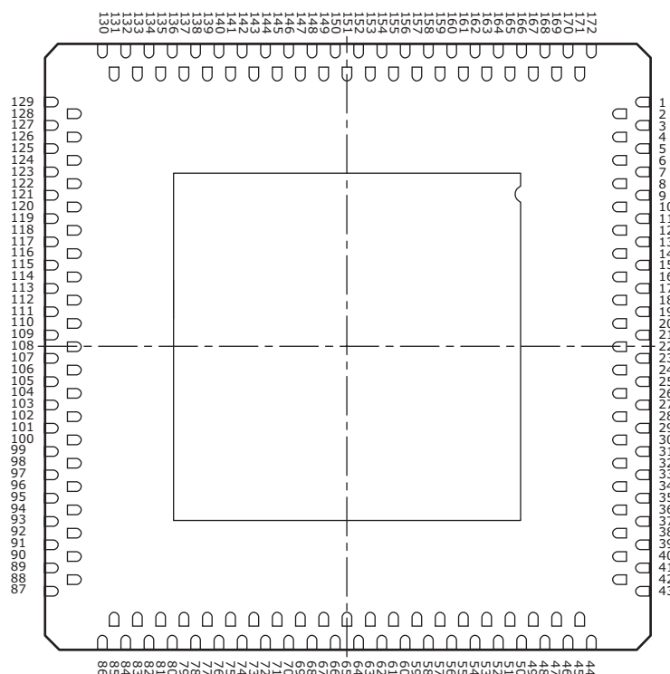
FIGURE 7-1: PIN DIAGRAM
