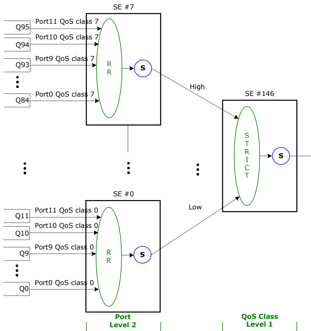
FIGURE 2-34: EGRESS SCHEDULER PORT 0
