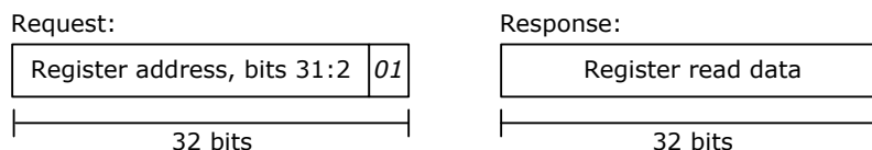
FIGURE 2-43: READ COMMAND
