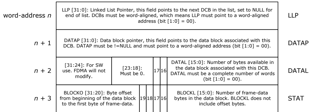
FIGURE 3-12: FDMA DCB LAYOUT
