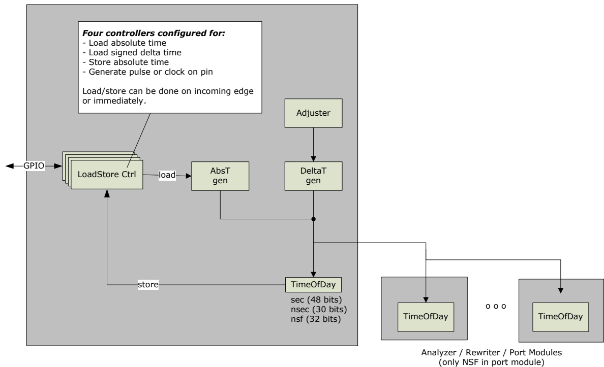
FIGURE 2-48: TIMING DISTRIBUTION
