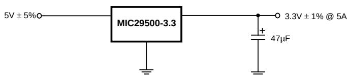
Figure 2. Using a Micrel LDO is very simple. Only an output filter capacitor is necessary. Here, 3.3V at 5A is produced from a nominal 5V input.
