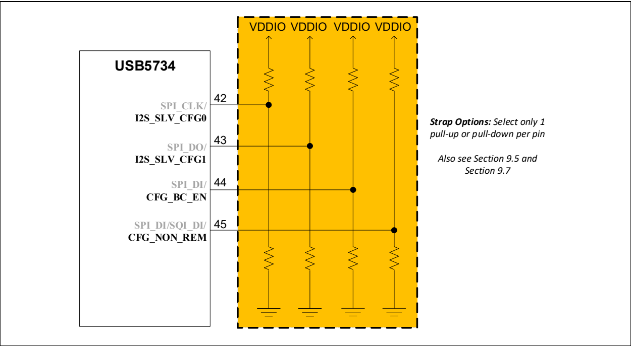
FIGURE 8-2: RECOMMENDED CONNECTIONS IF SPI FLASH IS NOT USED
