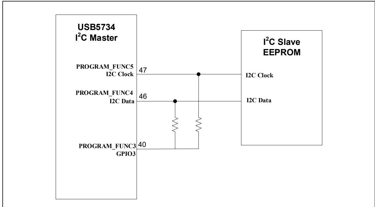
FIGURE 9-2: I 2 C MASTER INTERFACE CONNECTIONS
