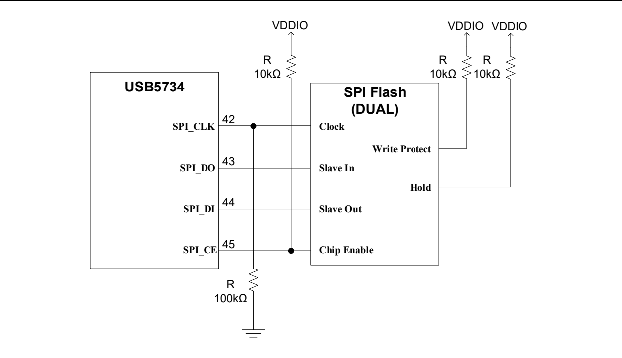
FIGURE 8-1: DUAL SPI FLASH CONNECTIONS
