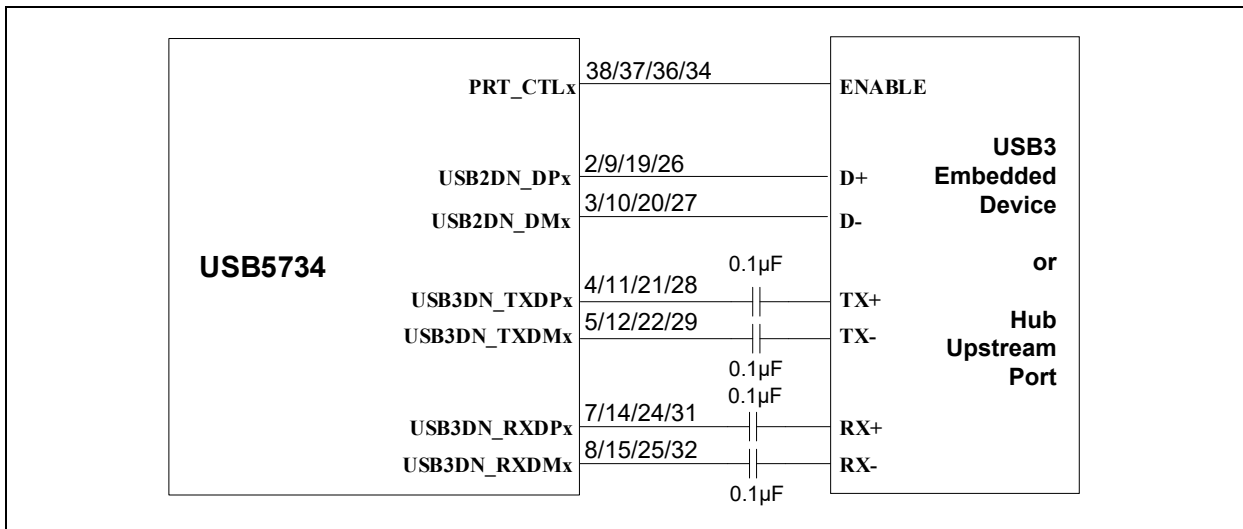
FIGURE 4-6: DOWNSTREAM PORT EMBEDDED DEVICE USB CONNECTIONS
