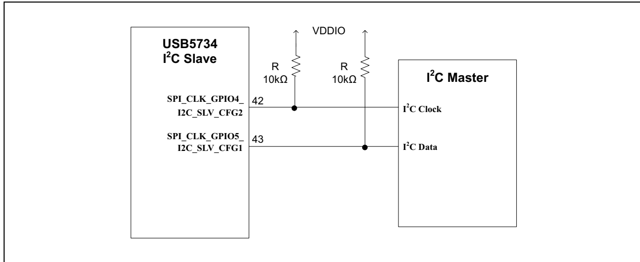
FIGURE 9-1: I 2 C SLAVE INTERFACE CONNECTIONS
