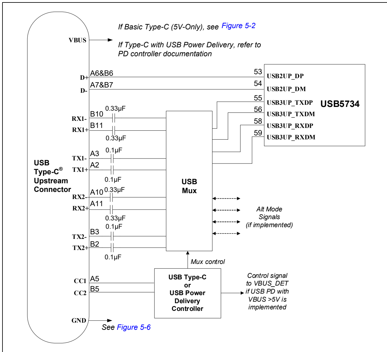
FIGURE 4-2: UPSTREAM PORT USB TYPE-C® USB CONNECTIONS
