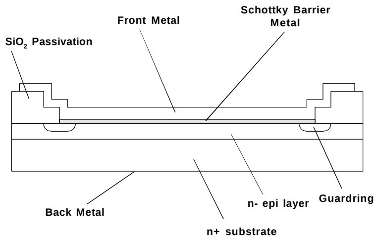
Figure 1 Vertical structure of Schottky Rectifier Die
