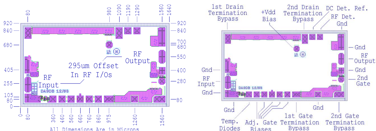
Figure 1. Die size, pad locations, and pad descriptions
