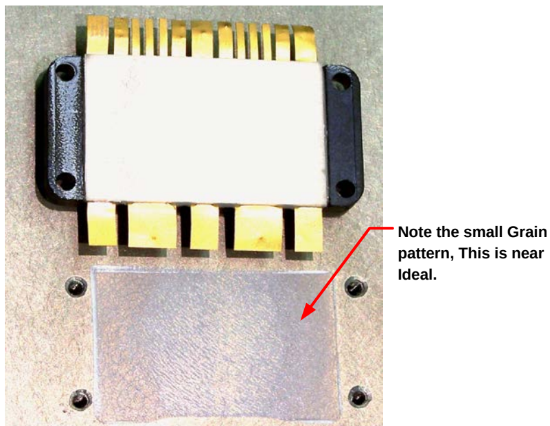
Figure 10 Uniform Coating of Thermal Grease
