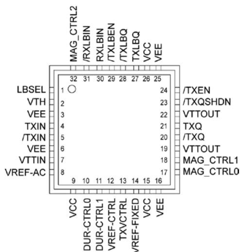
32-Pin QFN
