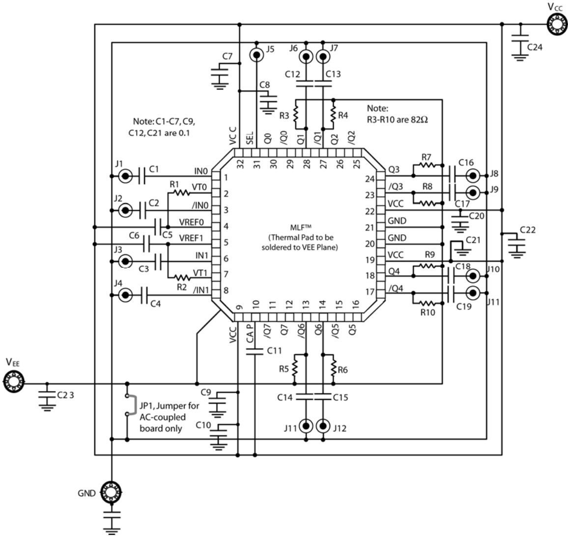
SY89837U AC-Coupled Evaluation Board
