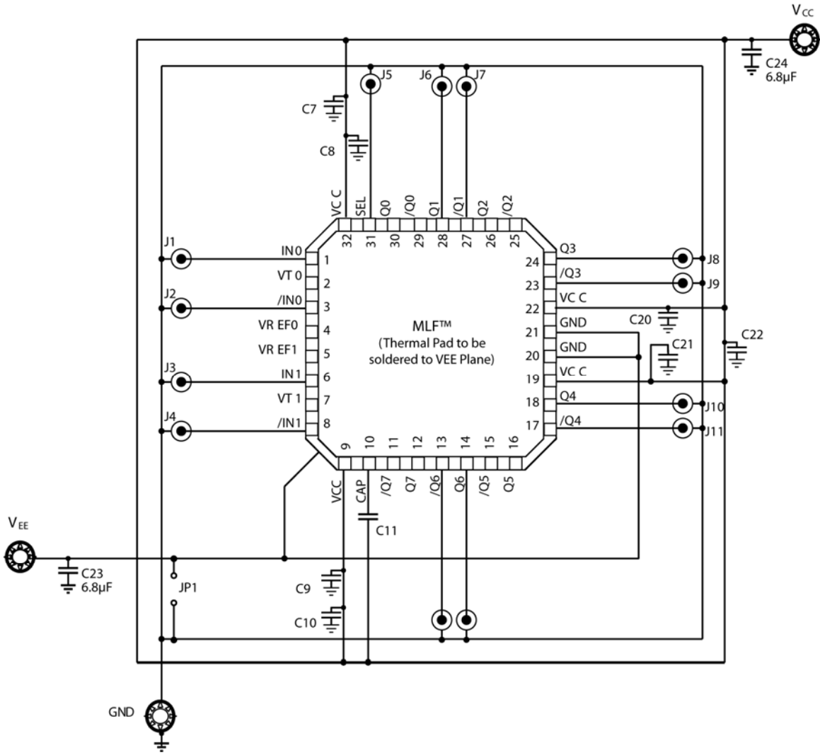
SY89837U DC-Coupled Evaluation Board
