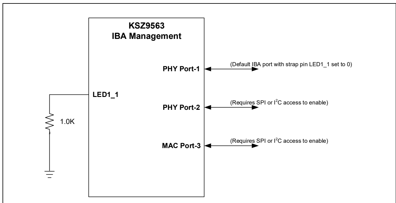
FIGURE 7-3: IBA BLOCK DIAGRAM
