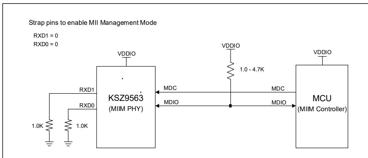
FIGURE 7-4: MII MANAGEMENT BLOCK DIAGRAM
