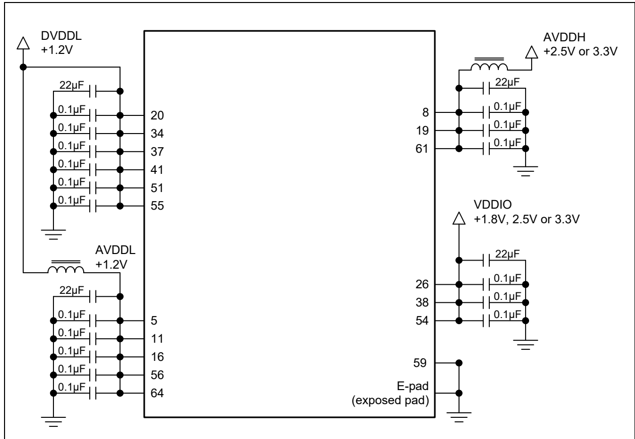
FIGURE 4-1: POWER AND GROUND CONNECTIONS
