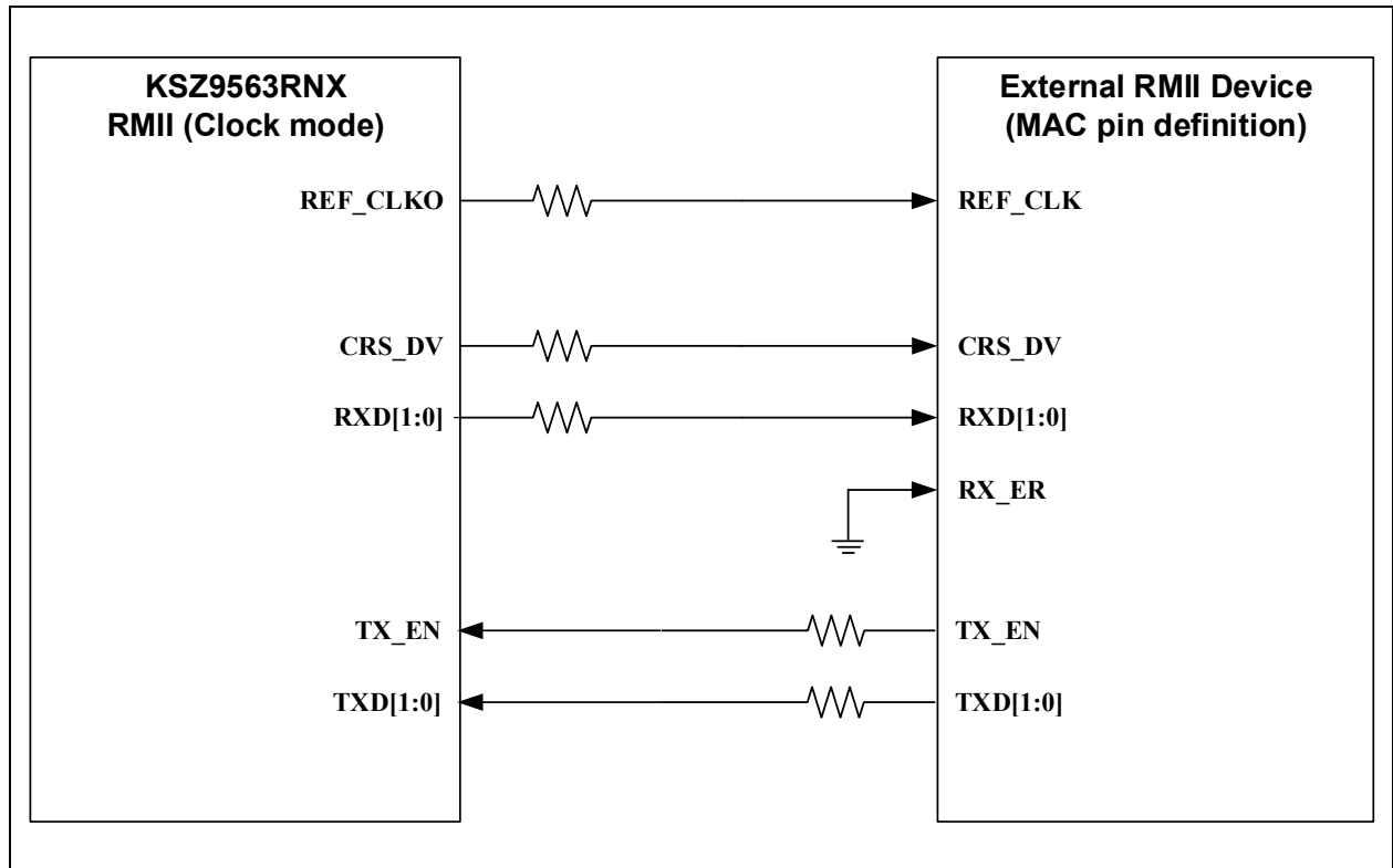
FIGURE 8-5: KSZ9563RNX RMII (CLOCK MODE) AND EXTERNAL RMII DEVICE (MAC PIN DEFINITION) - BLOCK DIAGRAM
