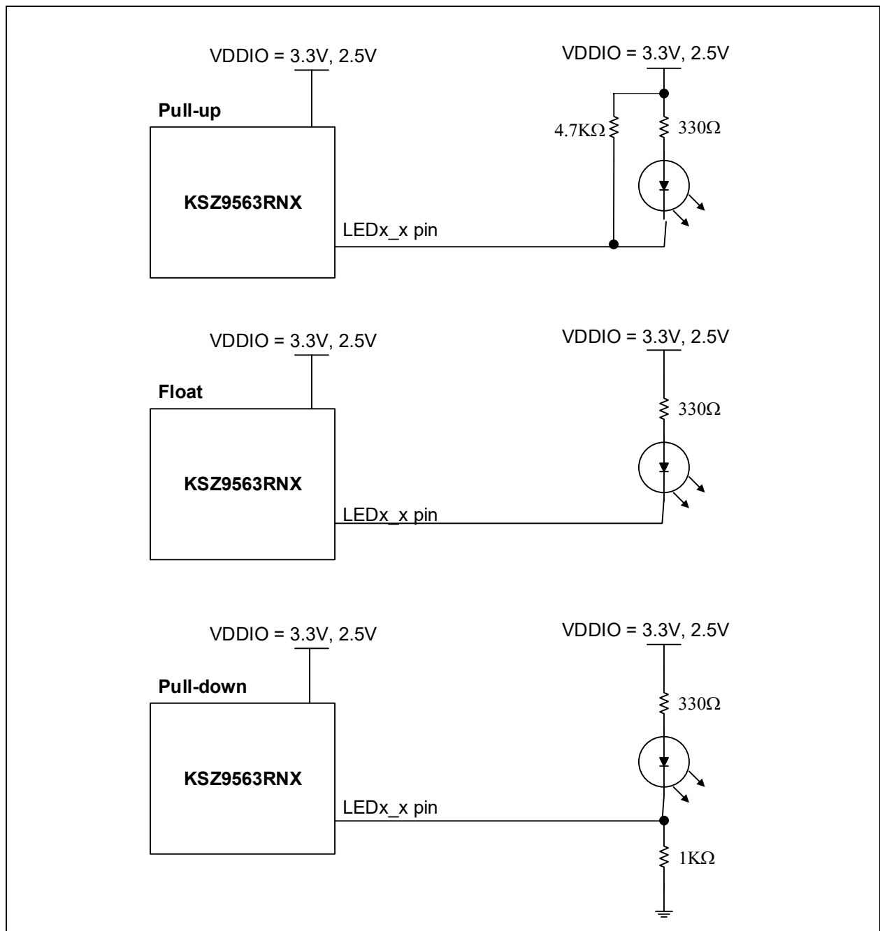
FIGURE 9-1: PHY Port LED Status and Pin Strapping - for VDDIO = 3.3V or 2.5V
