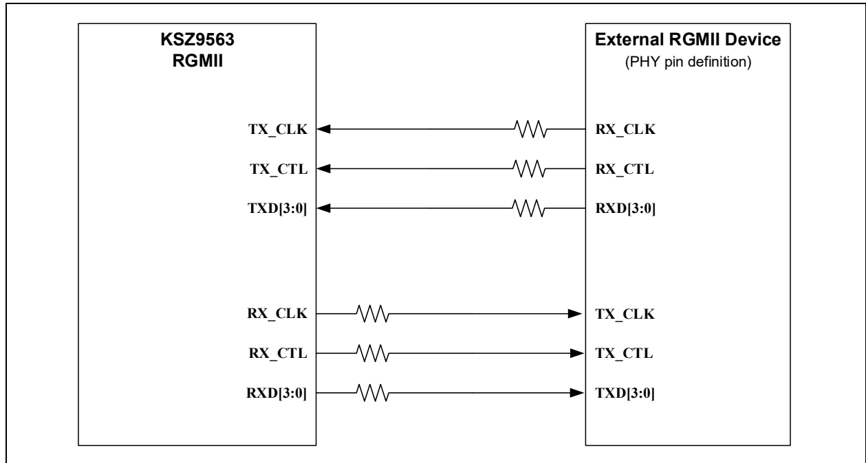
FIGURE 8-4: KSZ9563RNX RGMII AND EXTERNAL RGMII DEVICE (PHY PIN DEFINITION) - BLOCK DIAGRAM
