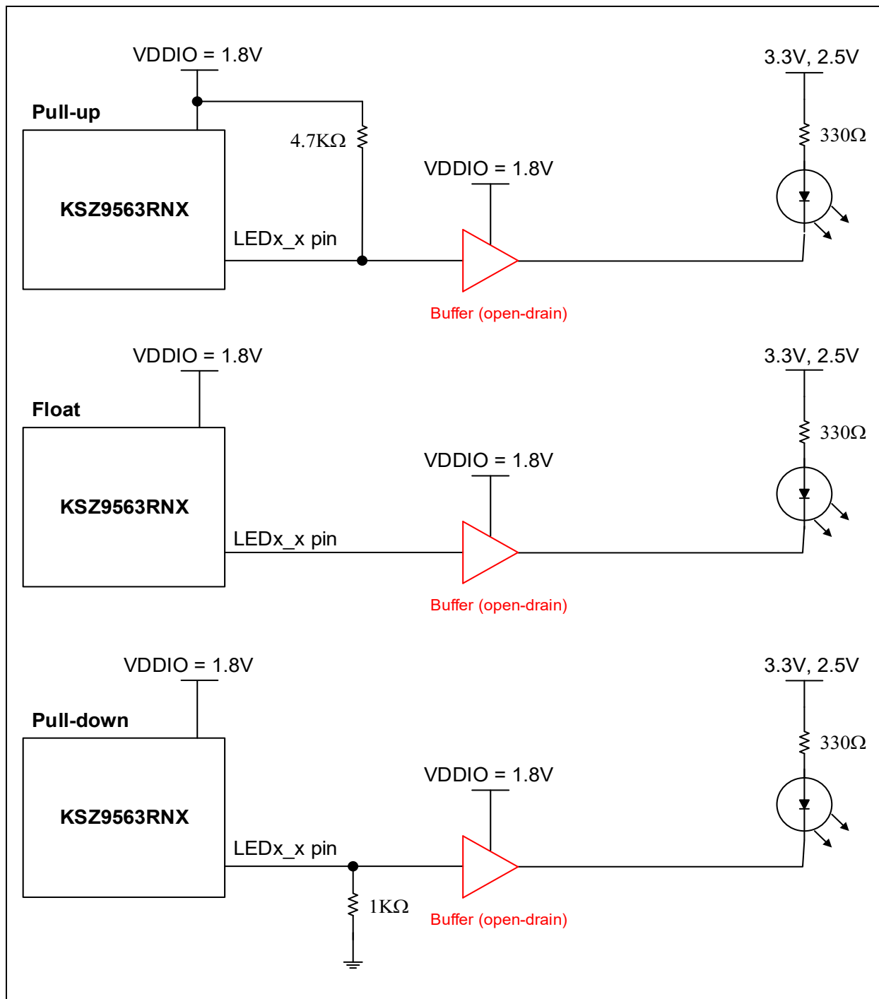
FIGURE 9-2: PHY Port LED Status and Pin Strapping - for VDDIO = 1.8V
