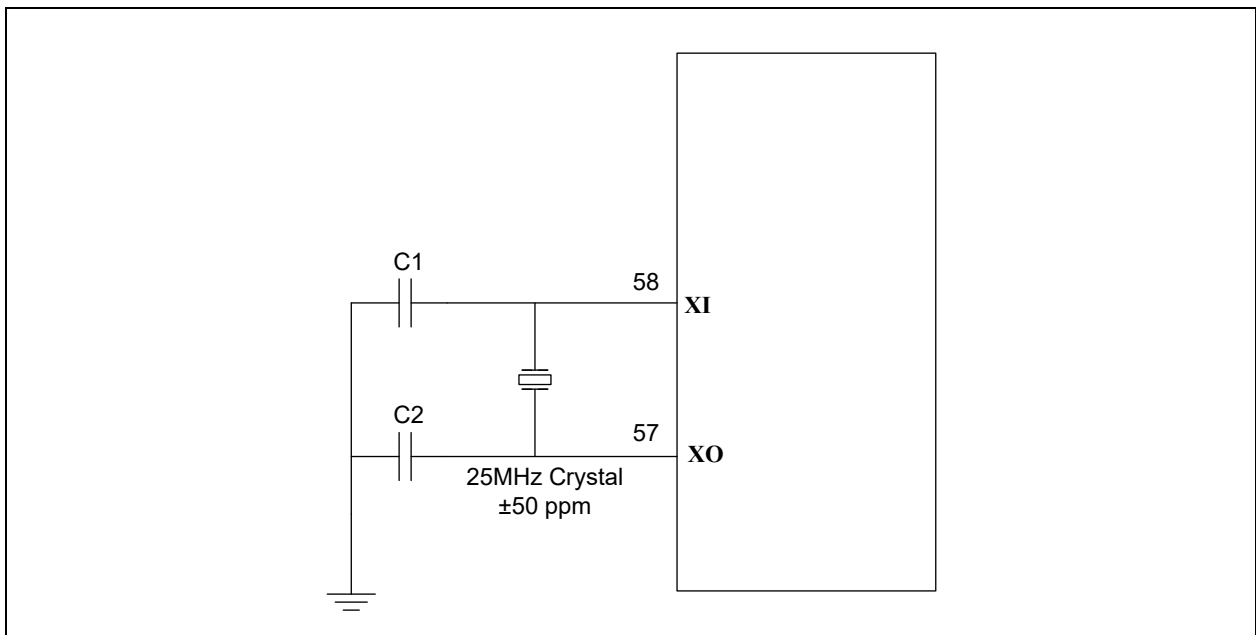
FIGURE 3-1: CRYSTAL CIRCUIT
