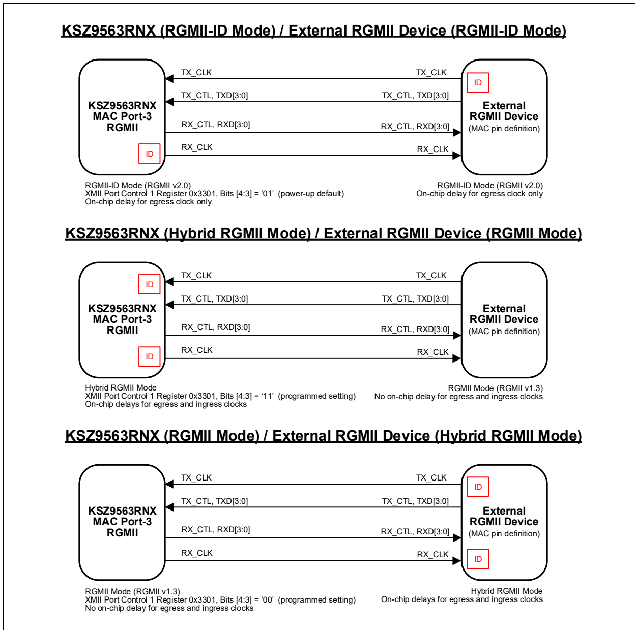
FIGURE 8-1: KSZ9563RNX AND EXTERNAL RGMII DEVICE (MAC PIN DEFINITION) - RGMII FUNCTIONAL CONFIGURATION WITH ON-CHIP CLOCK DELAY OPTIONS
