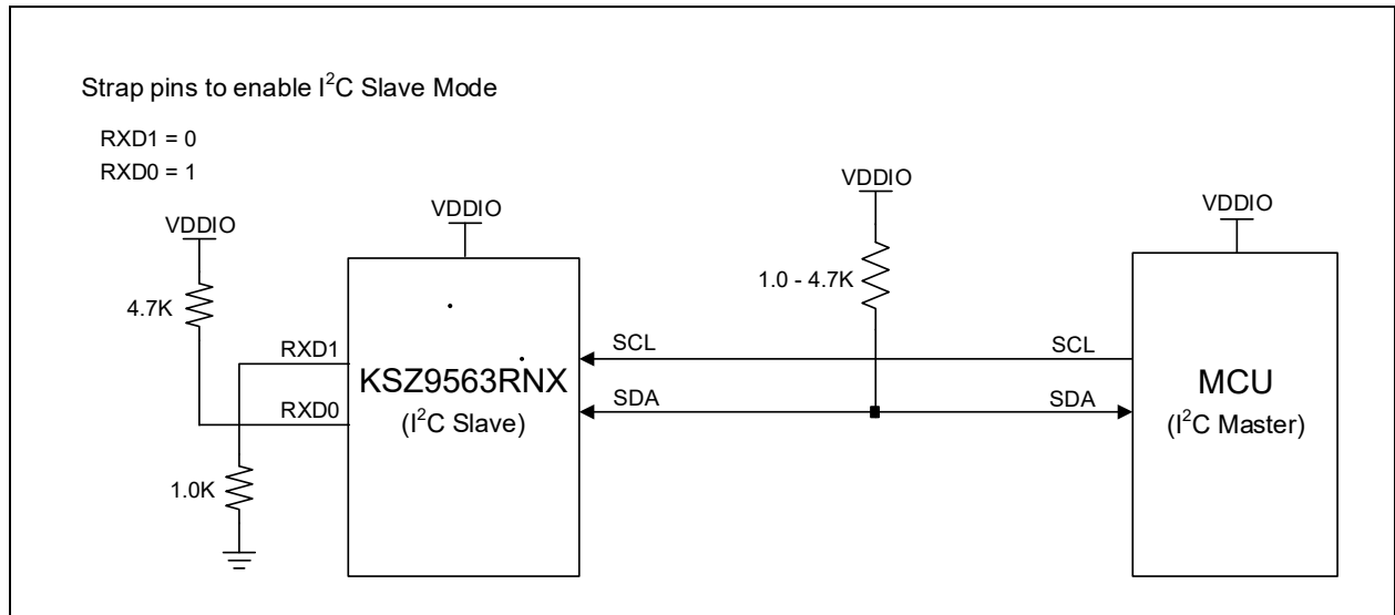
FIGURE 7-2: I 2 C BLOCK DIAGRAM
