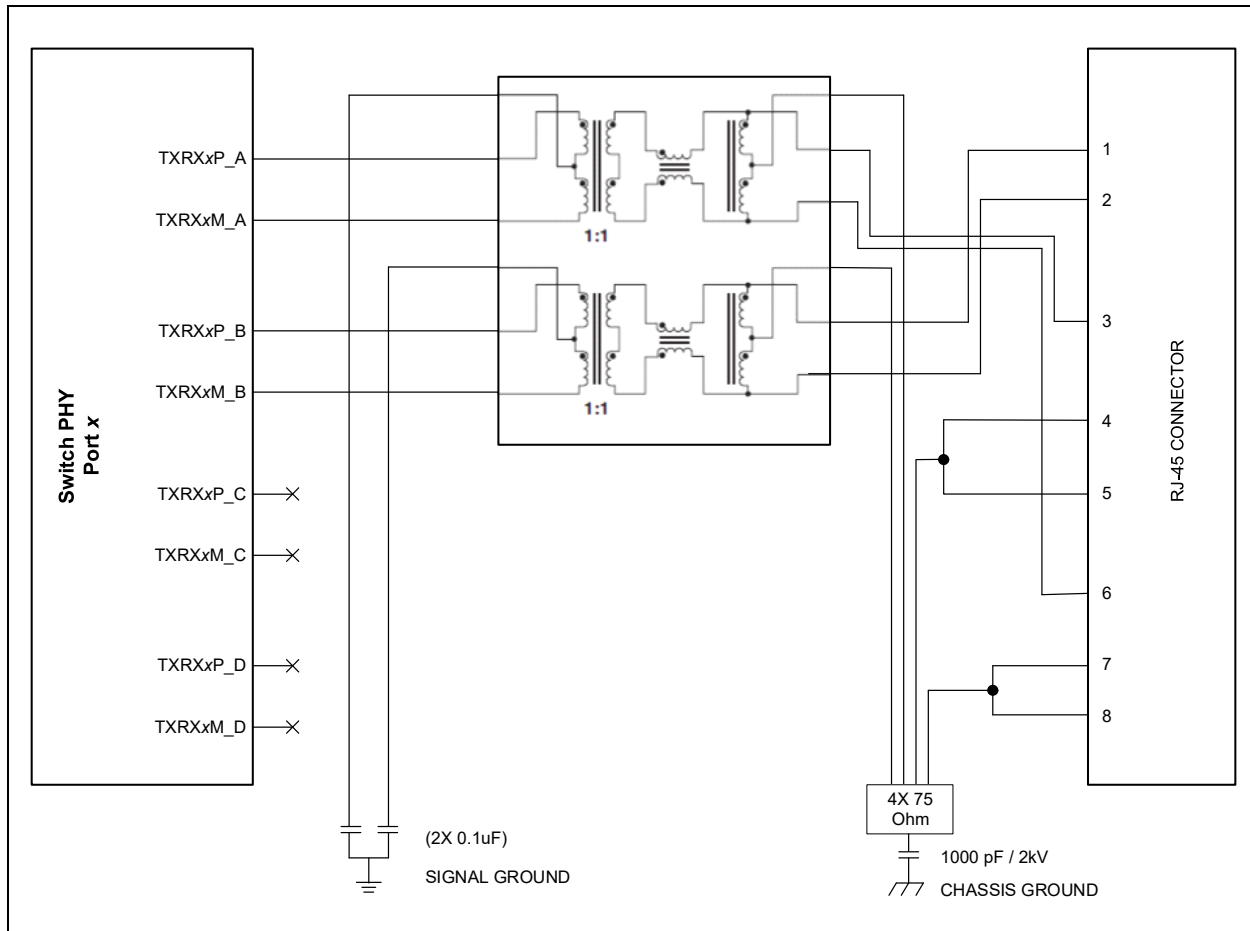
FIGURE 6-3: FAST ETHERNET MAGNETIC CONNECTIONS (MDI-X MODE)
