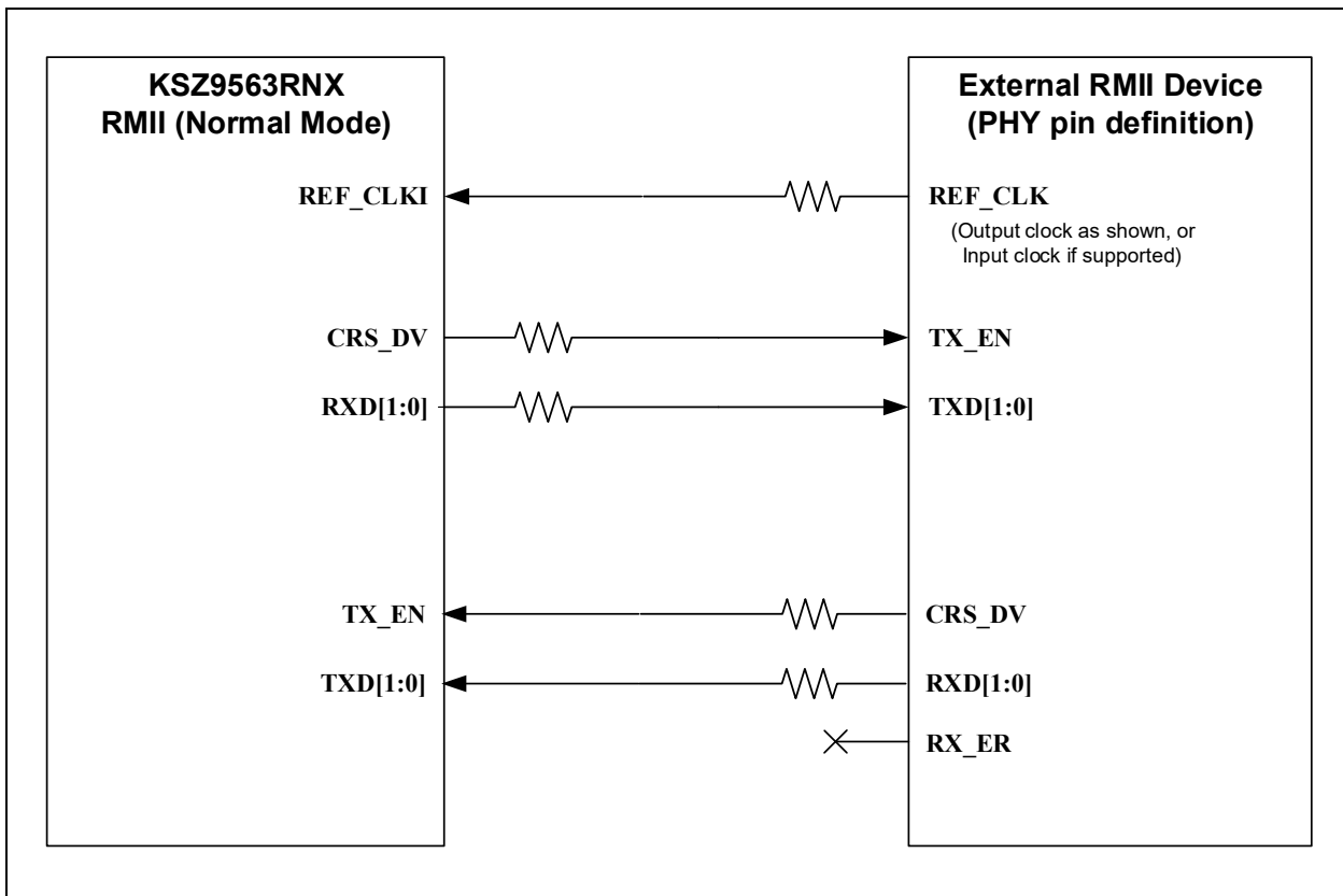
FIGURE 8-6: KSZ9563RNX RMII (NORMAL MODE) AND EXTERNAL RMII DEVICE (PHY PIN DEFINITION) - BLOCK DIAGRAM
