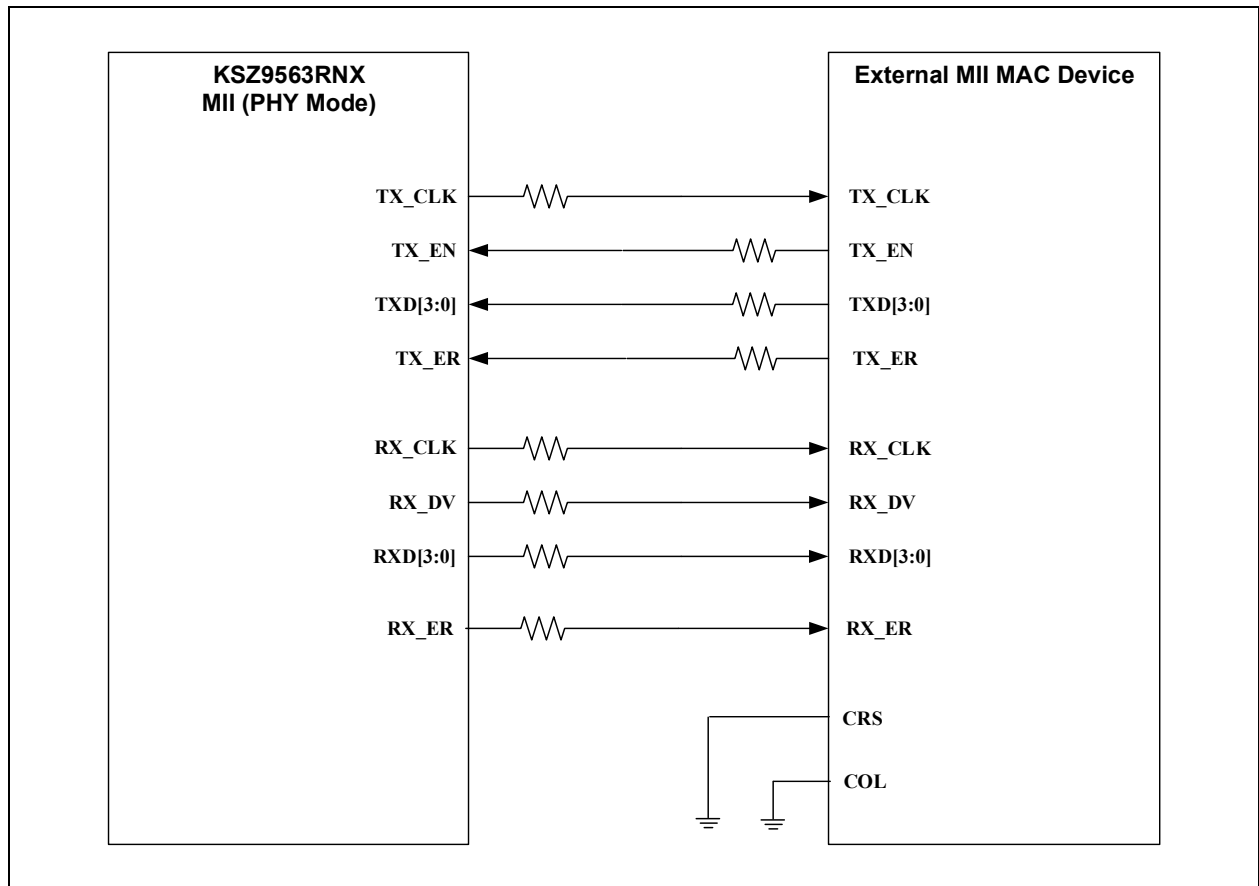
FIGURE 8-8: KSZ9563RNX MII (PHY MODE) AND EXTERNAL MII MAC - BLOCK DIAGRAM
