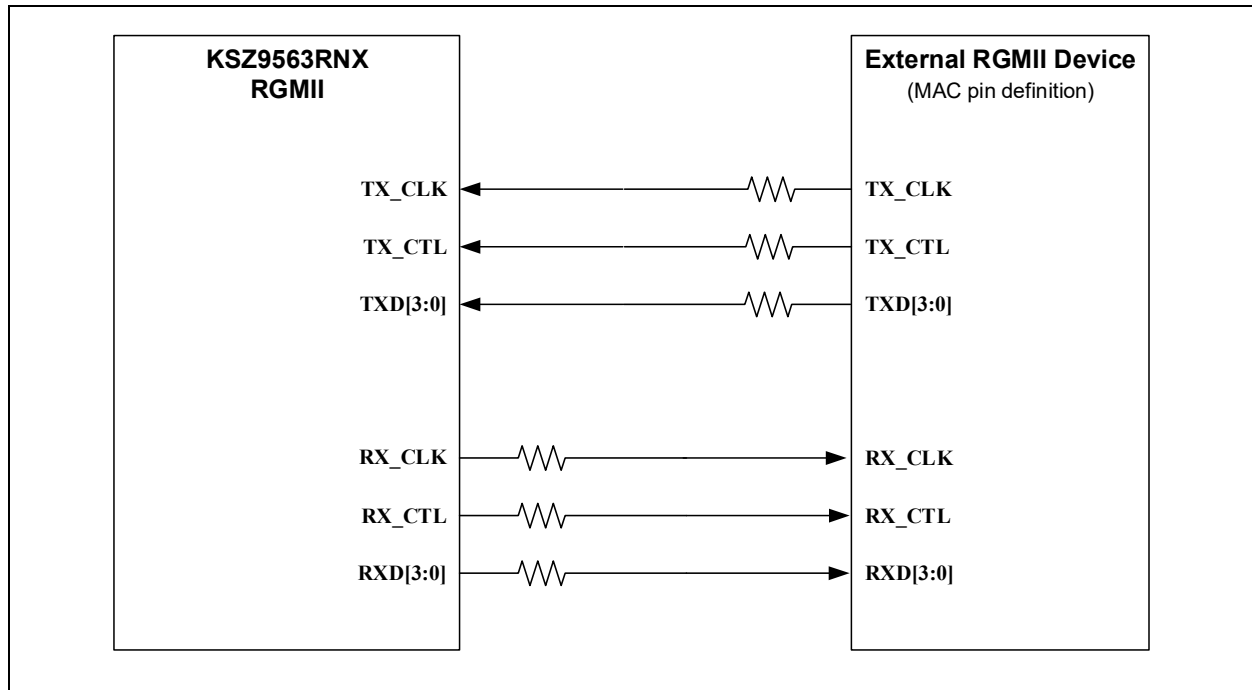
FIGURE 8-3: KSZ9563RNX RGMII AND EXTERNAL RGMII DEVICE (MAC PIN DEFINITION) - BLOCK DIAGRAM
