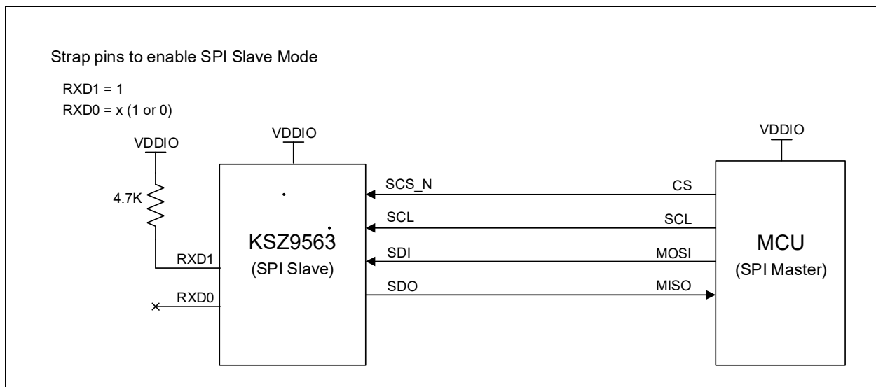
FIGURE 7-1: SPI BLOCK DIAGRAM
