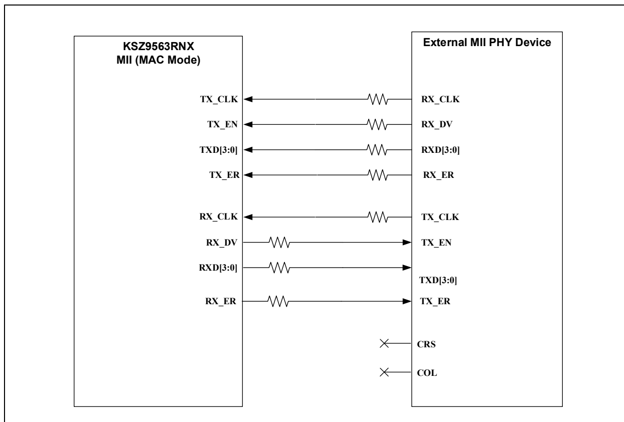
FIGURE 8-7: KSZ9563RNX MII (MAC MODE) AND EXTERNAL MII PHY - BLOCK DIAGRAM
