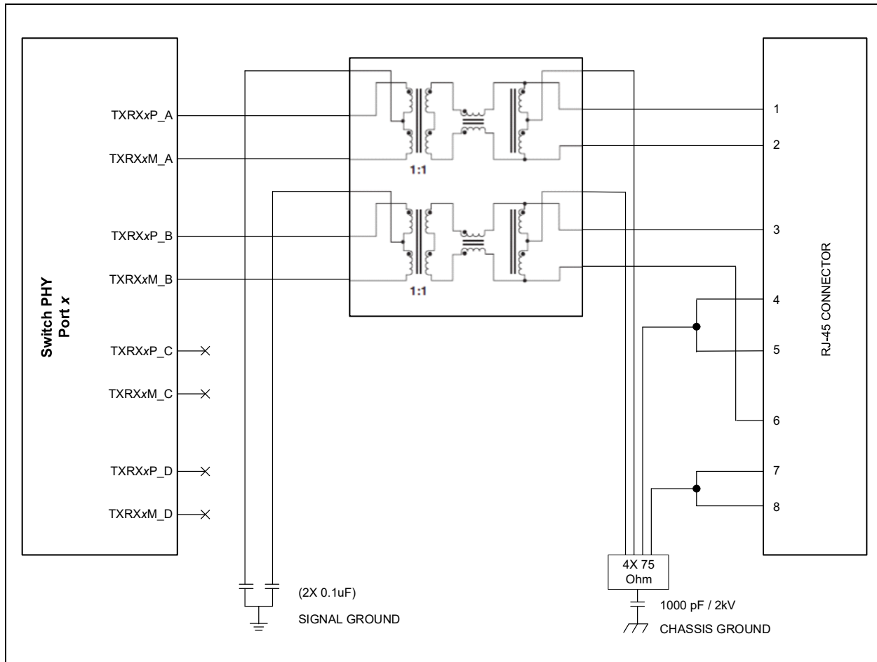
FIGURE 6-2: FAST ETHERNET MAGNETIC CONNECTIONS (MDI MODE)
