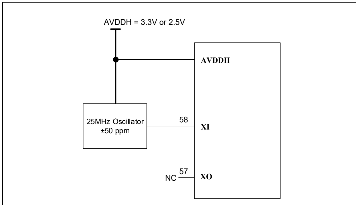
FIGURE 3-2: EXTERNAL CLOCK SOURCE/OSCILLATOR CIRCUIT
