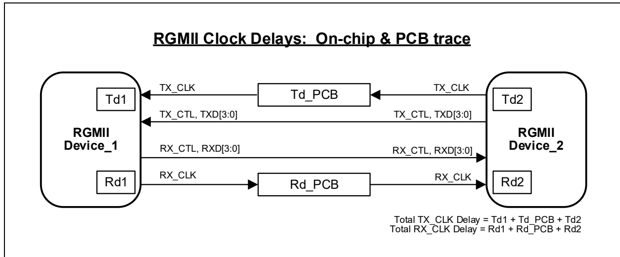
FIGURE 8-2: RGMII CLOCK SKEW DIAGRAM
