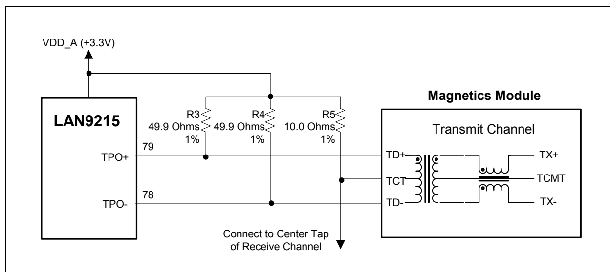
Figure 2.1 Transmit Circuit
