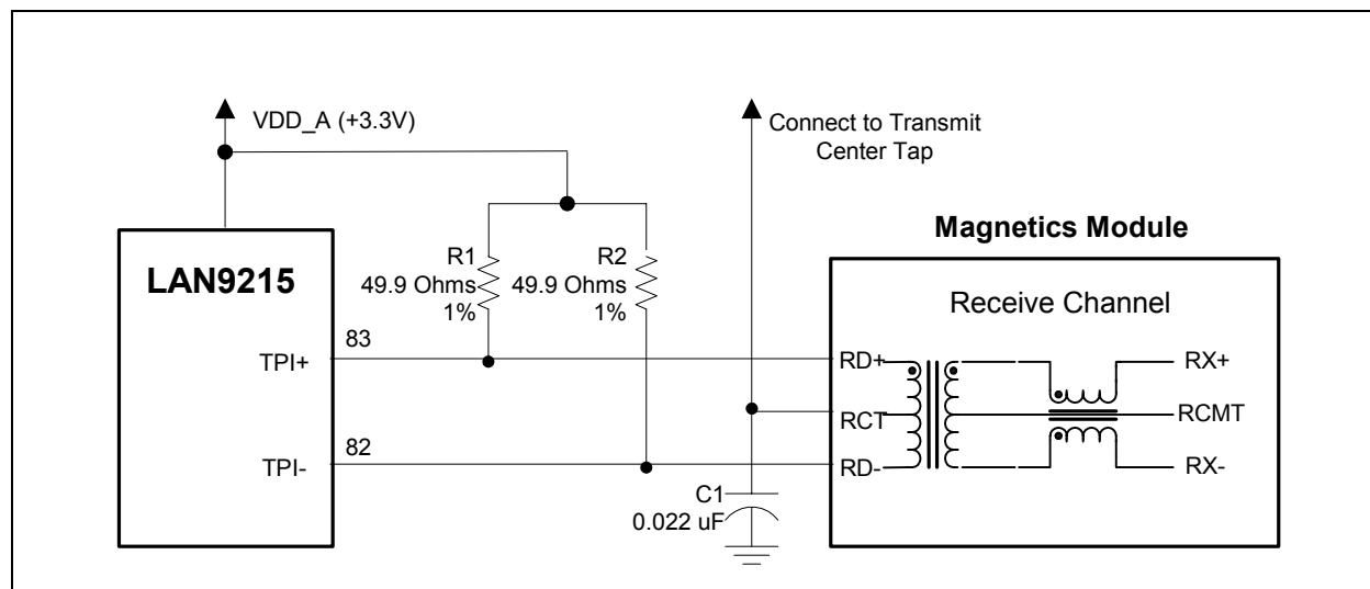
Figure 2.2 Receive Circuit
