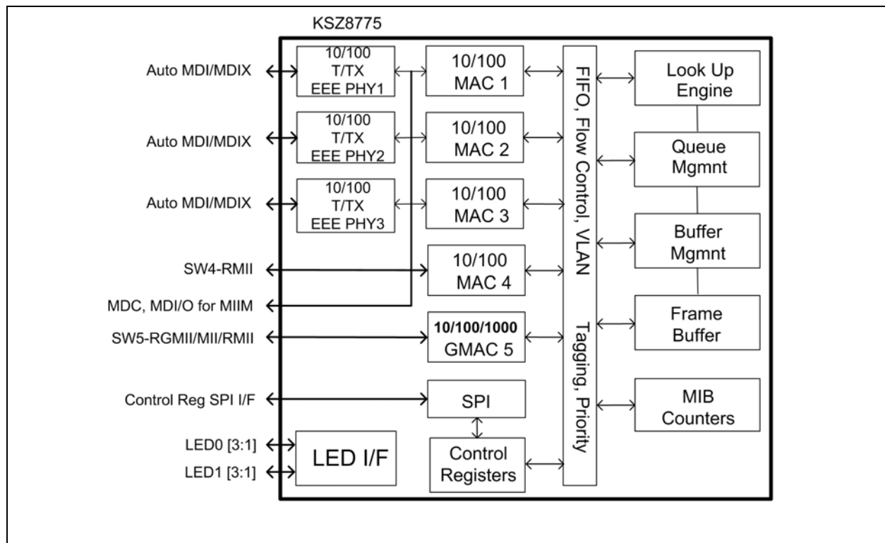
FIGURE 1-1: BLOCK DIAGRAM
