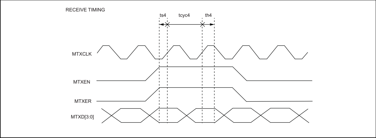
FIGURE 7-5: PHY MODE MII TIMING – DATA TRANSMITTED FROM MII
