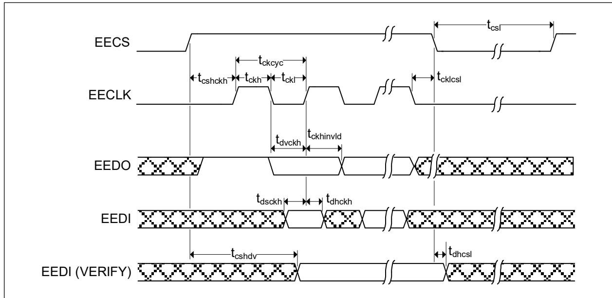
FIGURE 7-5: EEPROM TIMING
