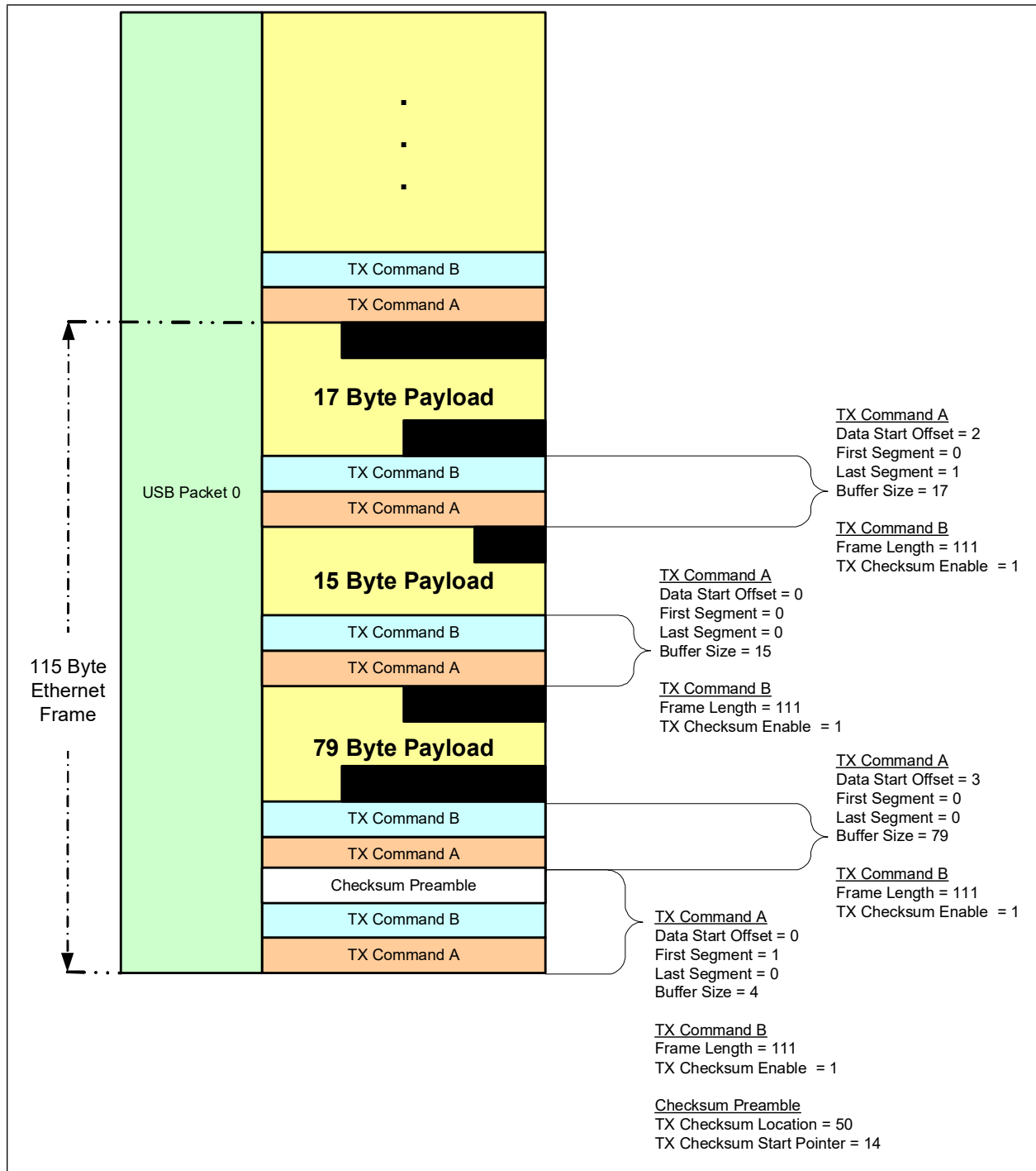
FIGURE 4-8: TX EXAMPLE 3
