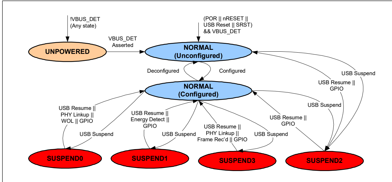
FIGURE 4-29: POWER STATES
