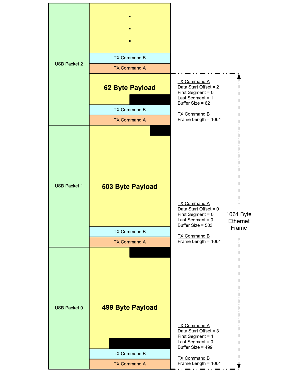
FIGURE 4-6: TX EXAMPLE 1
