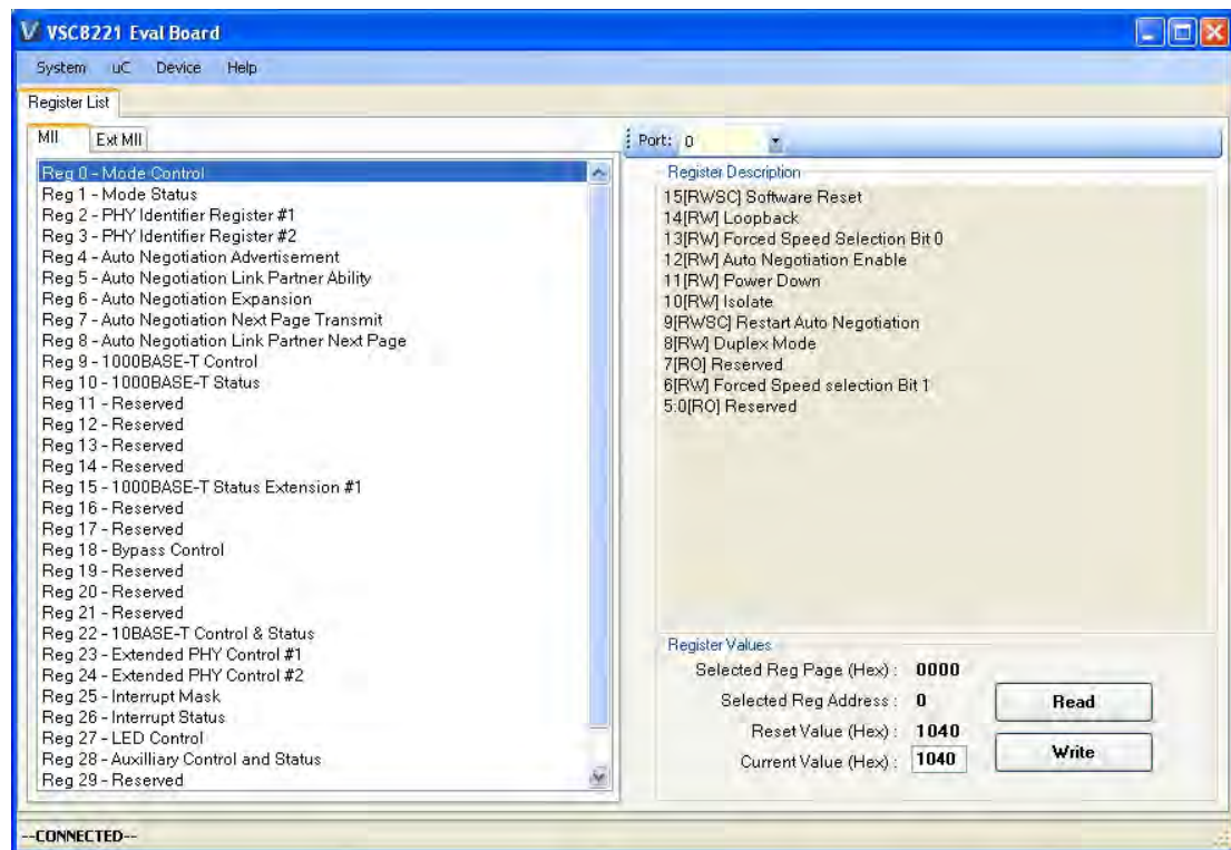
Figure 4 • Register List Window
