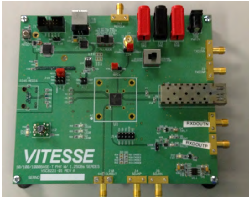
Figure 1 • VSC8221EV
