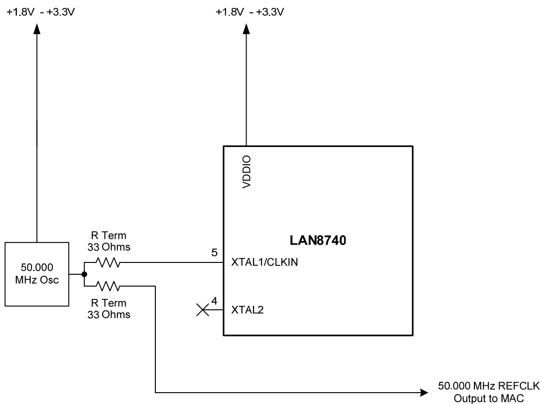
Figure 5 – LAN8740 Clock Oscillator Connections
