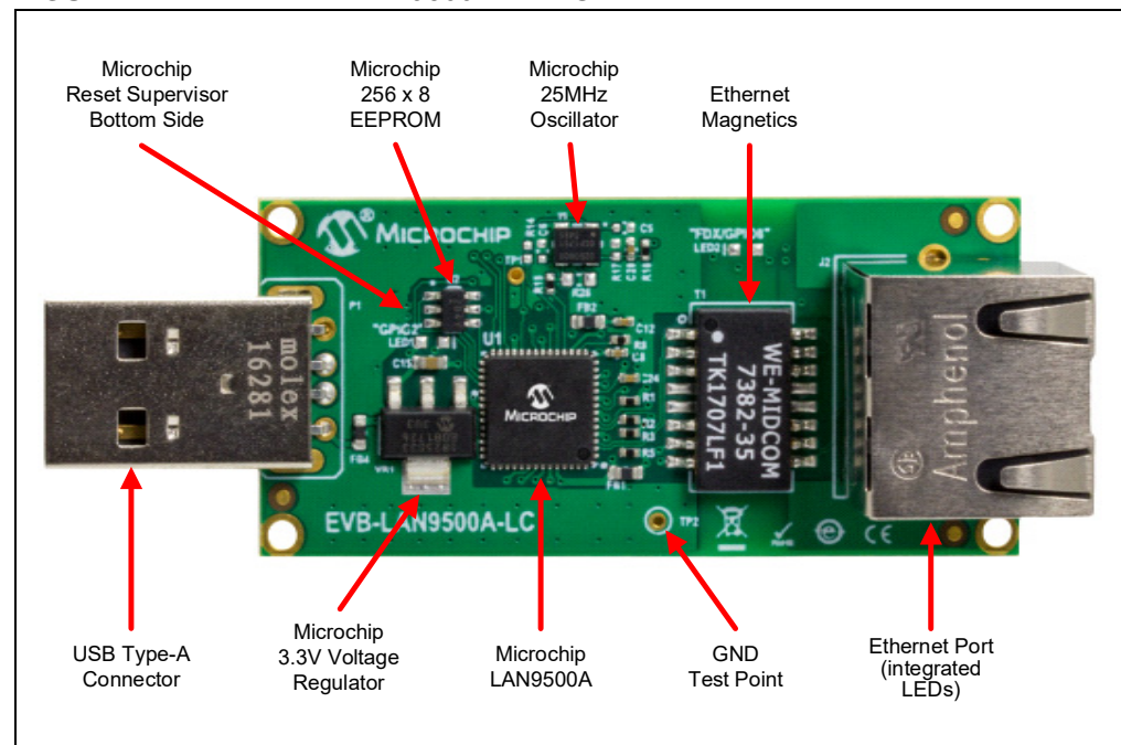
FIGURE 2-1: EVB-LAN9500A-LC TOP VIEW
