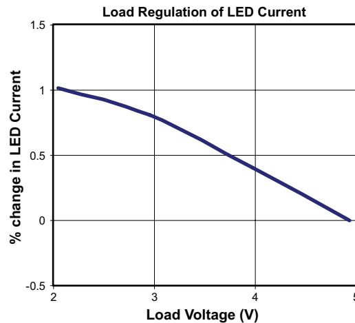
Fig. 4. Load Regulation of LED Current Plot
