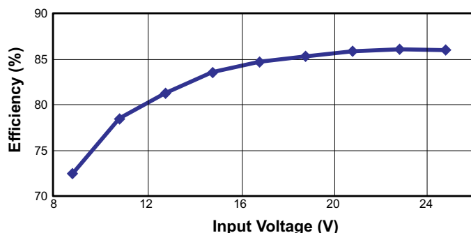
Fig. 1. Efficiency vs Input Voltage
