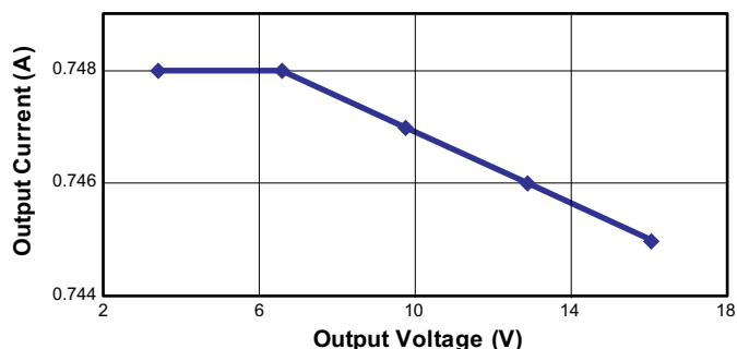
Fig. 3. Load Regulation of the Output Current
