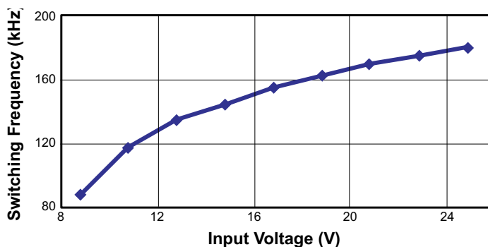
Fig. 4. Switching Frequency Regulation
