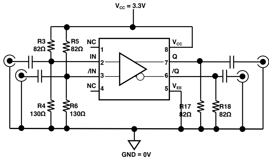
SY89327L AC-Coupled Evaluation Board
