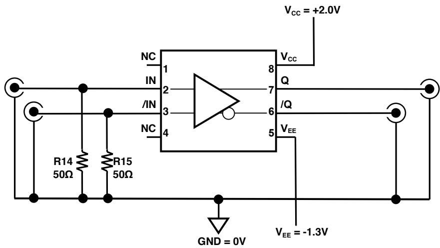
SY89327L DC-Coupled Evaluation Board
