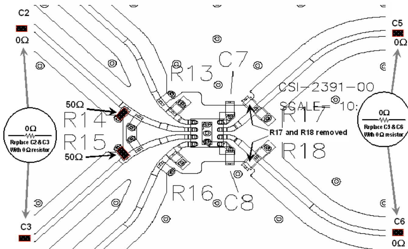
SY89327L DC-Coupled Loading Diagram
