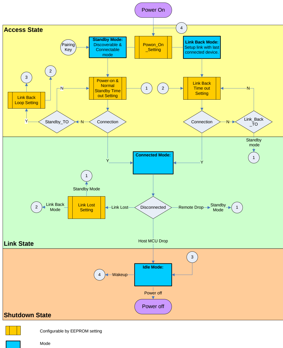
Fig2. IS1678S State Machine Diagram
