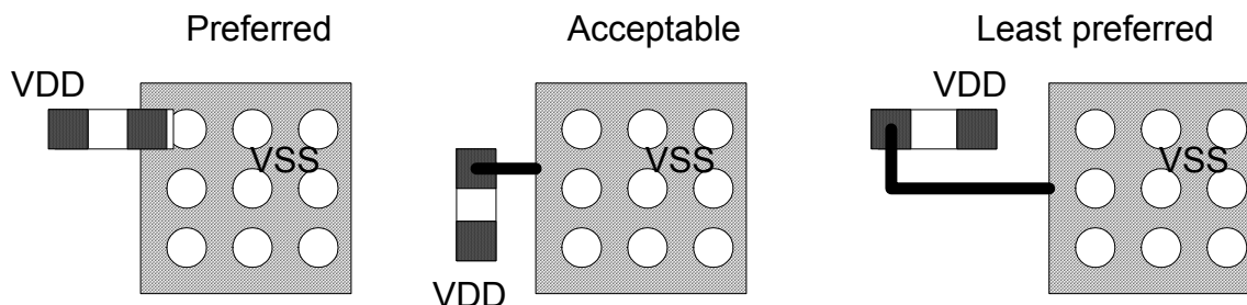
Figure 2.5 Placement of Bypass Capacitors
