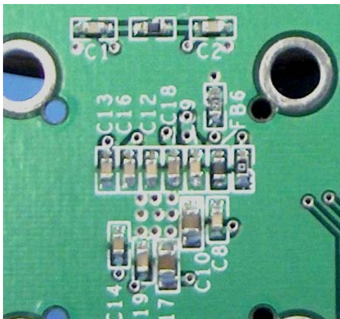
Figure 2.4 Crystal Oscillator Component Layout
