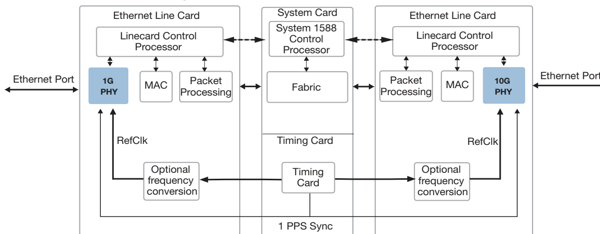
Figure 19 • IEEE 1588 Block Diagram
