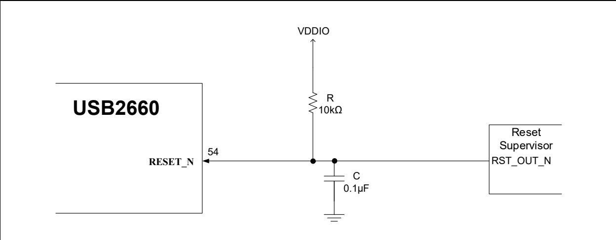
FIGURE 7-2: RESET CIRCUIT INTERFACE WITH CPU/MCU RESET OUTPUT
