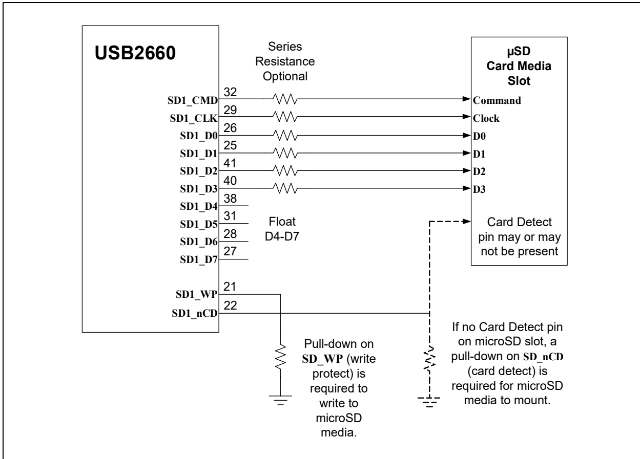
FIGURE 5-3: MICROSD CARD SLOT CONNECTIONS
