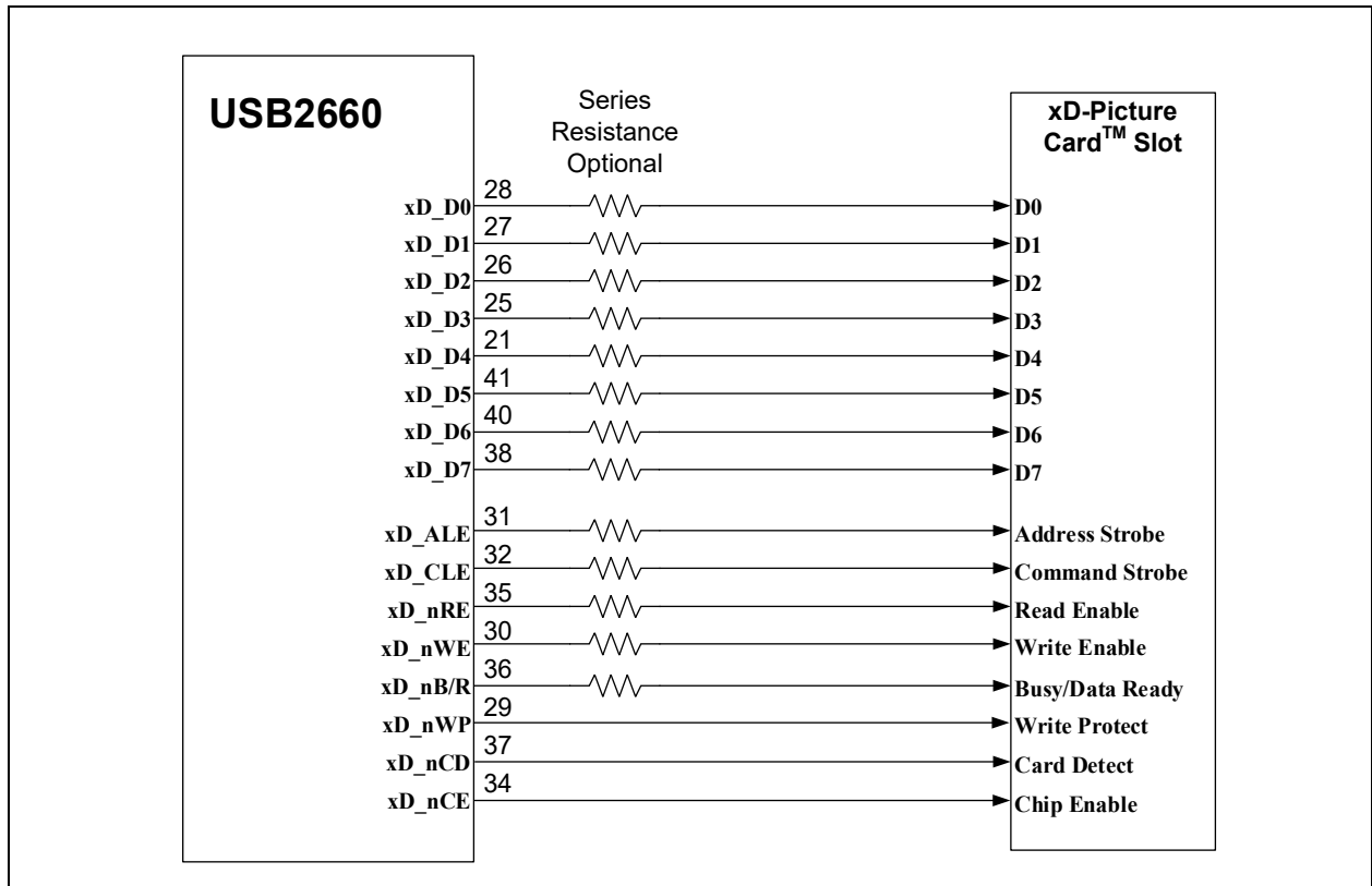
FIGURE 5-5: XD-PICTURE CARD™ SLOT CONNECTIONS
