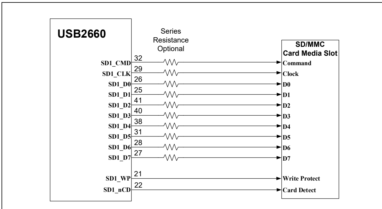
FIGURE 5-1: SD/MMC MEDIA SLOT 1
