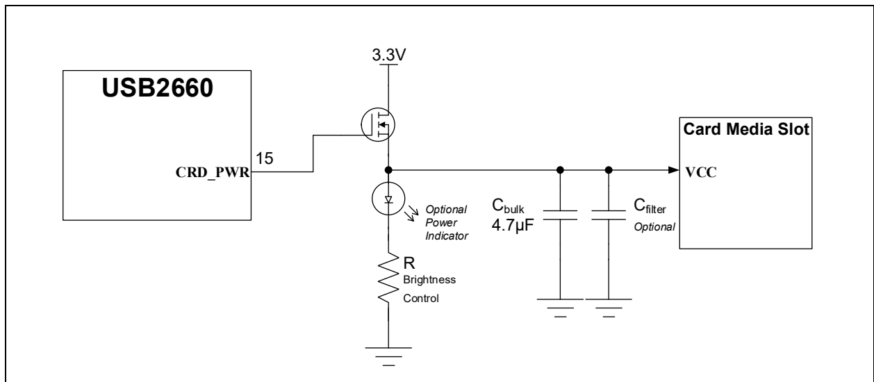
FIGURE 5-8: EXTERNAL CARD POWER SUPPLY SWITCH RECOMMENDED CONNECTIONS
