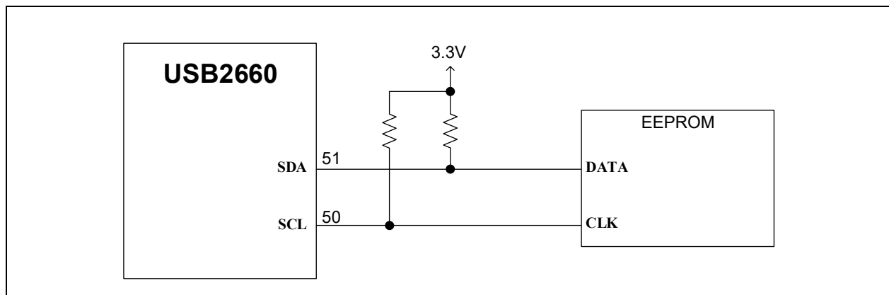
FIGURE 8-1: EEPROM CONNECTIONS
