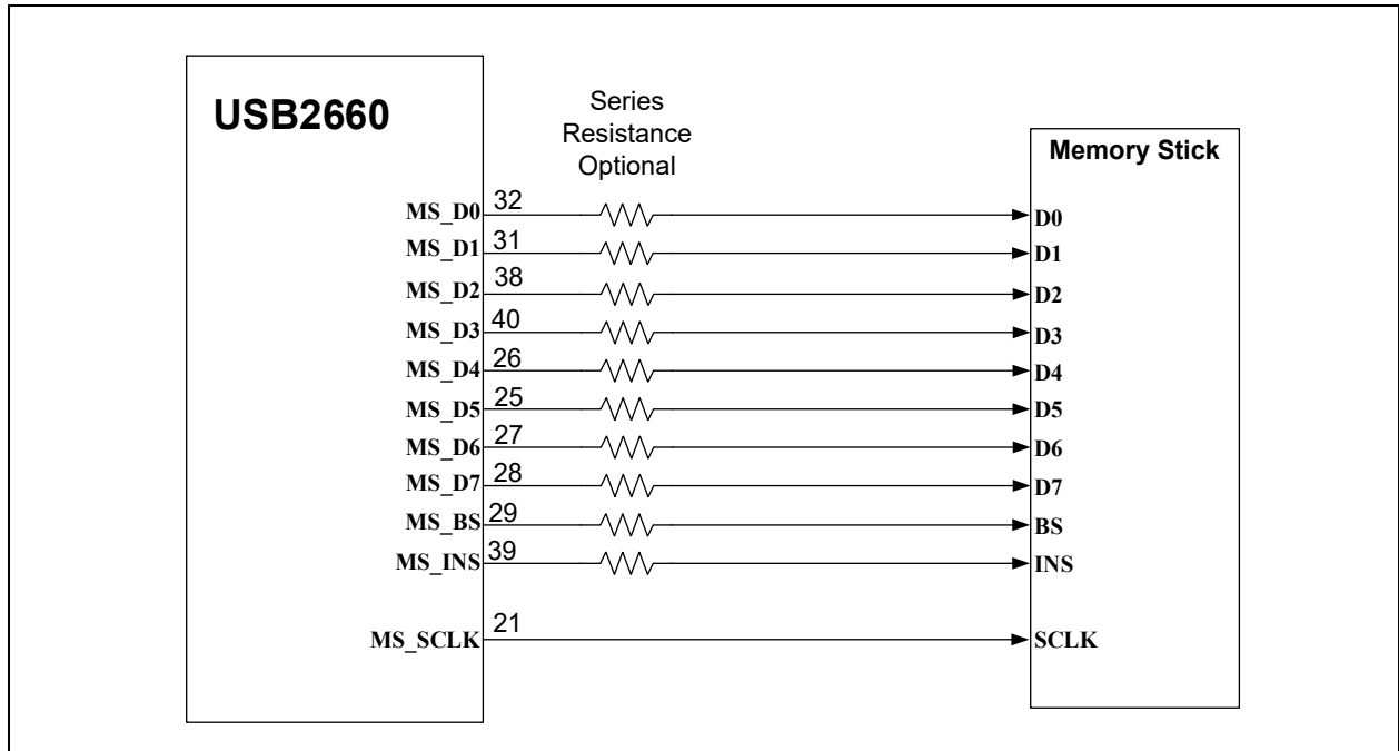
FIGURE 5-4: MEMORY STICK® CARD SLOT CONNECTIONS
