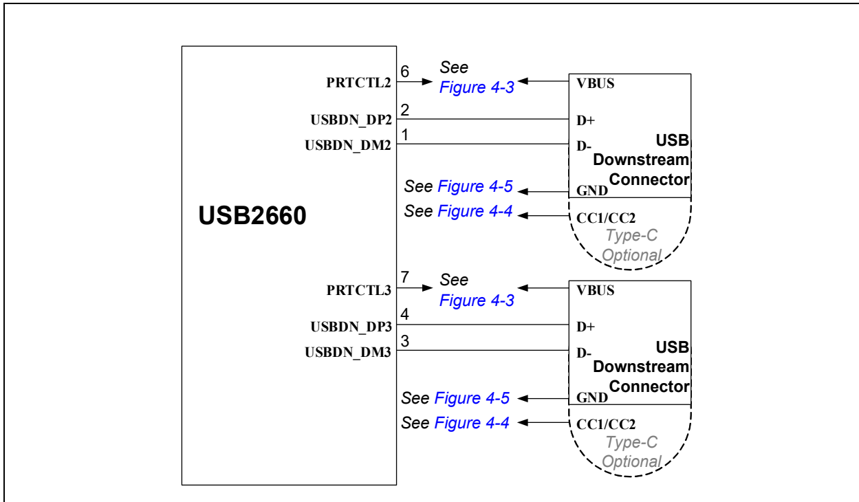
FIGURE 4-2: USB DOWNSTREAM PORT DATA SIGNAL CONNECTIONS
