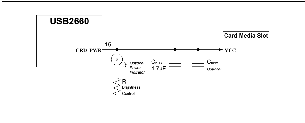
FIGURE 5-7: CRD_PWR CARD MEDIA POWER SUPPLY SWITCH
