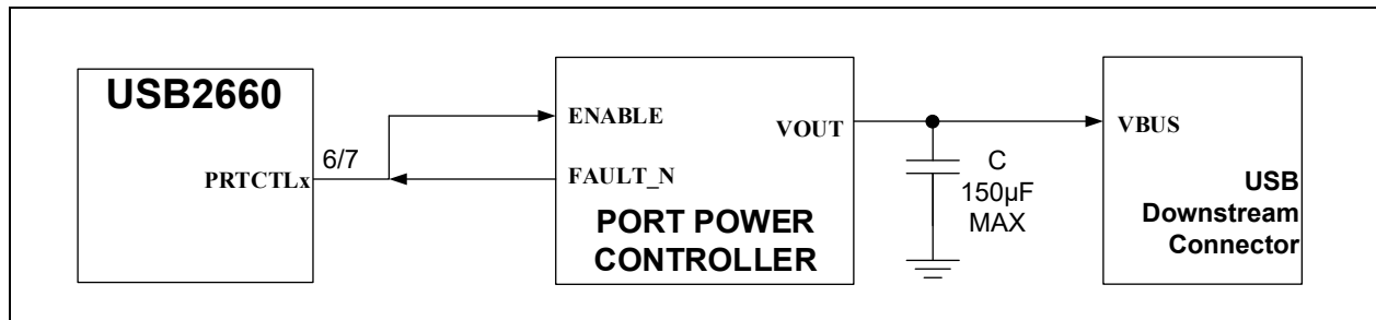
FIGURE 4-3: DOWNSTREAM VBUS AND PRTCTL1 CONNECTIONS
