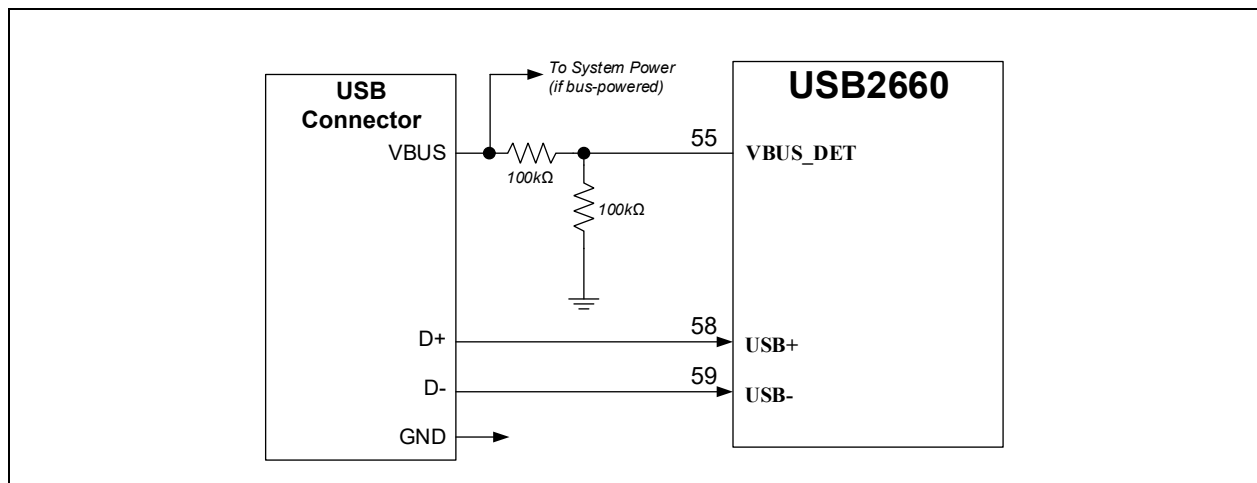
FIGURE 4-1: USB DATA SIGNAL CONNECTIONS
