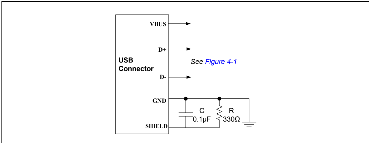
FIGURE 4-5: RECOMMENDED USB CONNECTOR GND AND SHIELD CONNECTIONS
