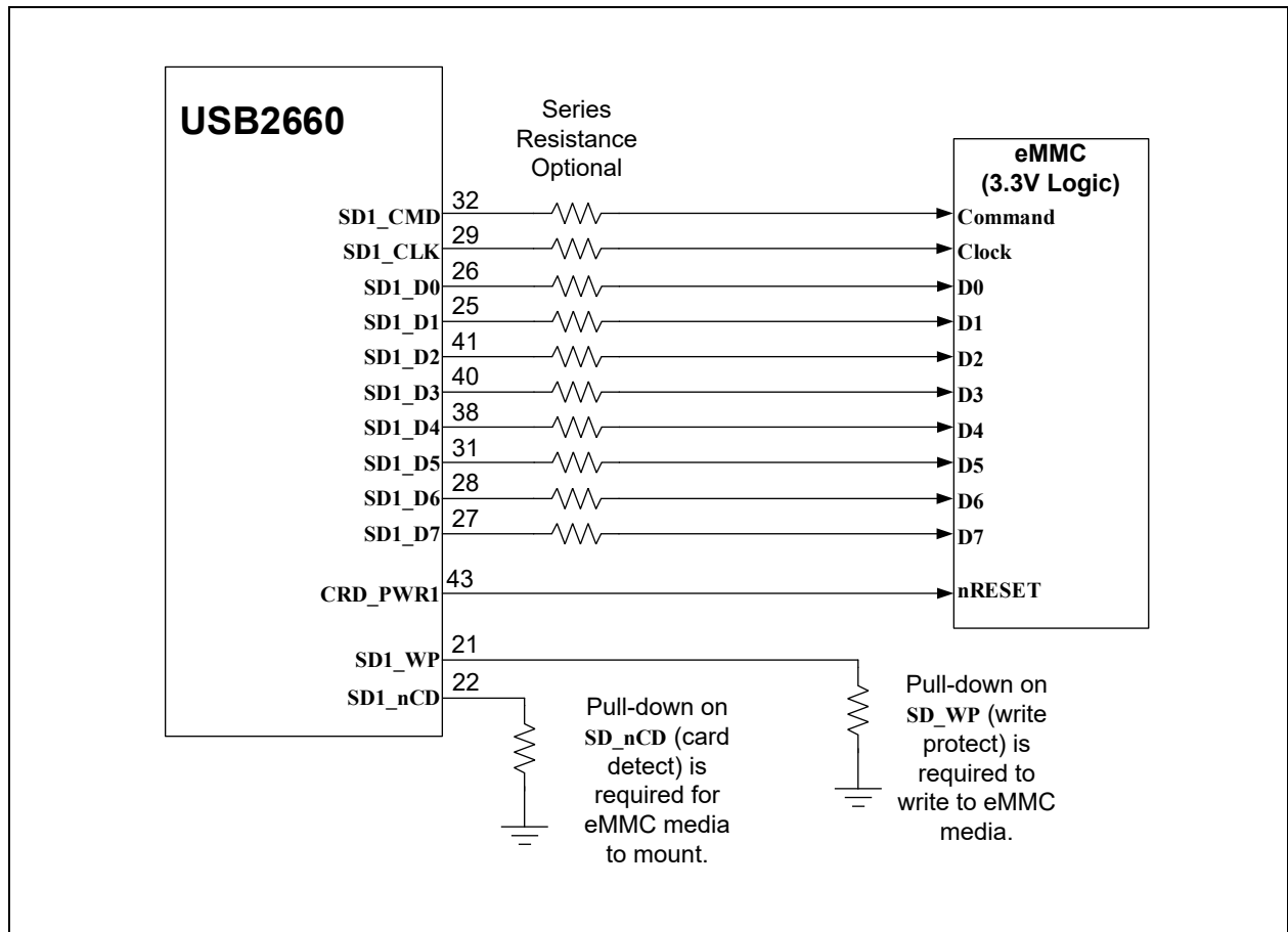
FIGURE 5-2: eMMC MEMORY CONNECTIONS
