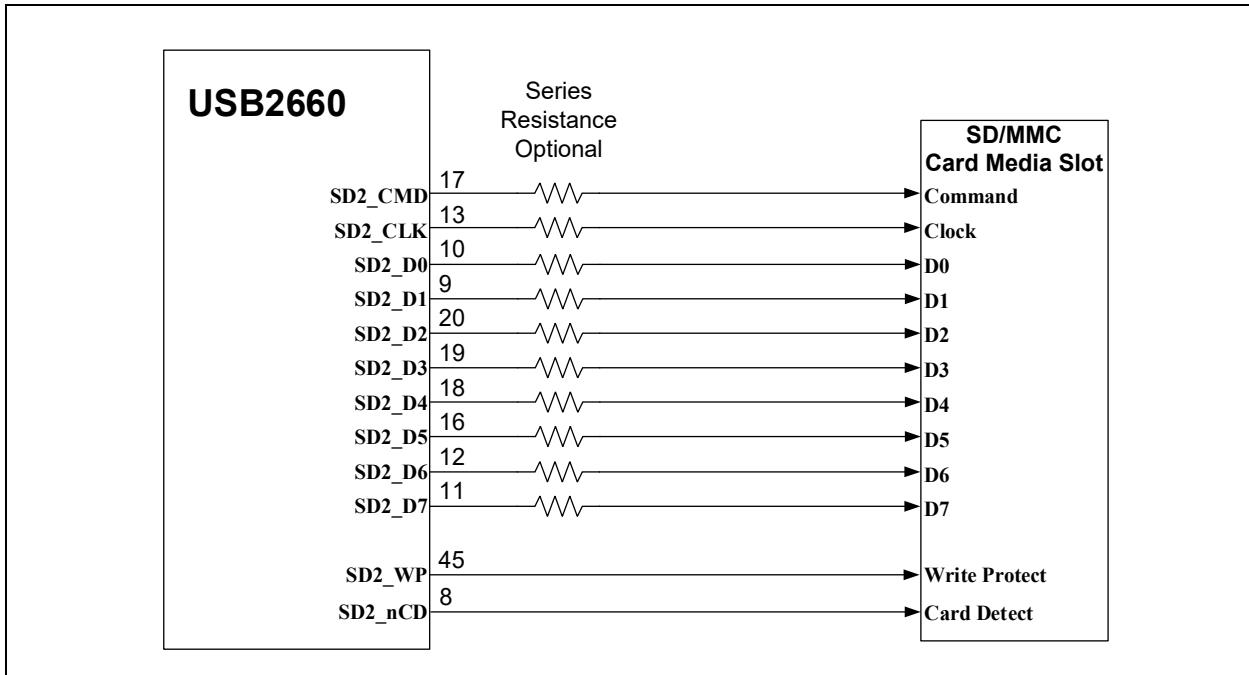
FIGURE 5-6: SD CARD SLOT 2 CONNECTIONS
