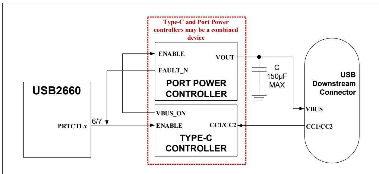
FIGURE 4-4: DOWNSTREAM VBUS AND PRTCTL1 CONNECTIONS WITH A TYPE-C PORT
