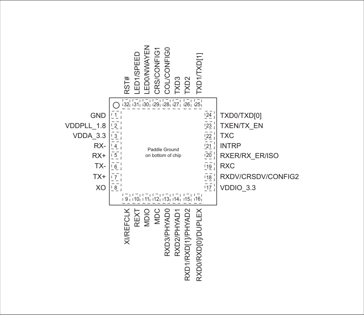
FIGURE 2-1: KSZ8041NL 32-VQFN PIN ASSIGNMENT (TOP VIEW)
