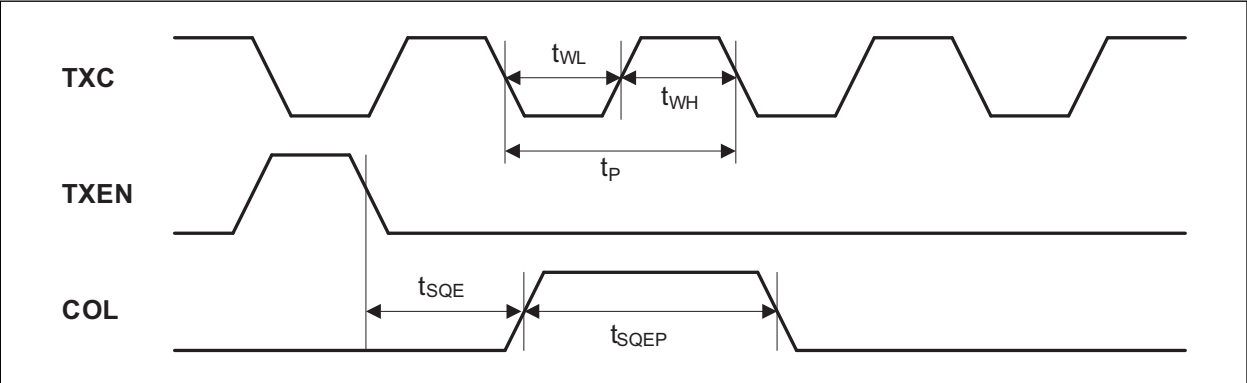
FIGURE 7-1: MII SQE TIMING (10BASE-T)
