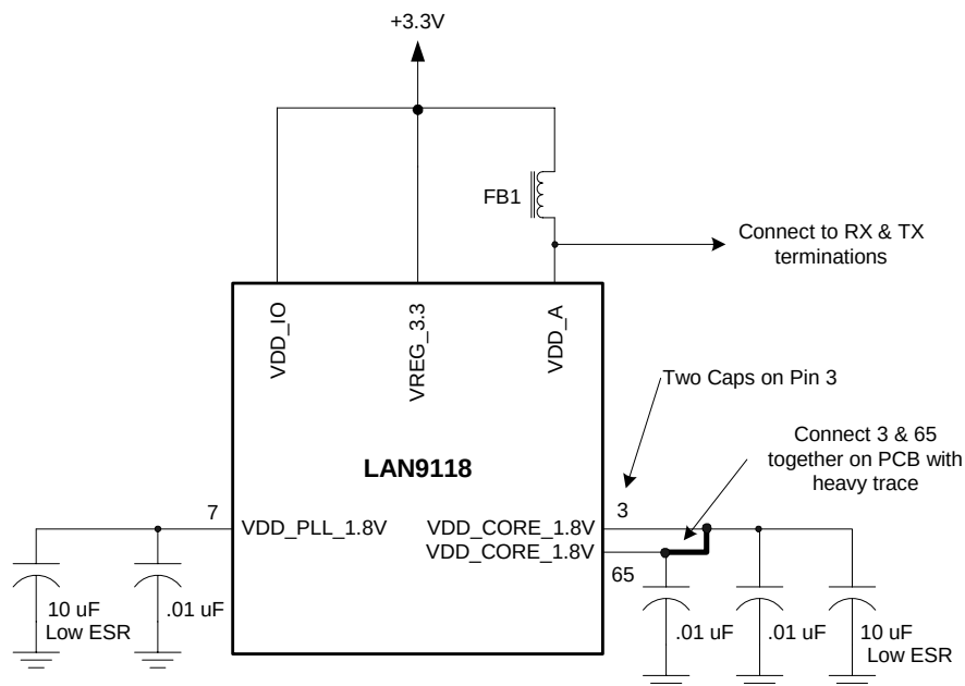
Figure 3 - LAN9118 Power Connections
