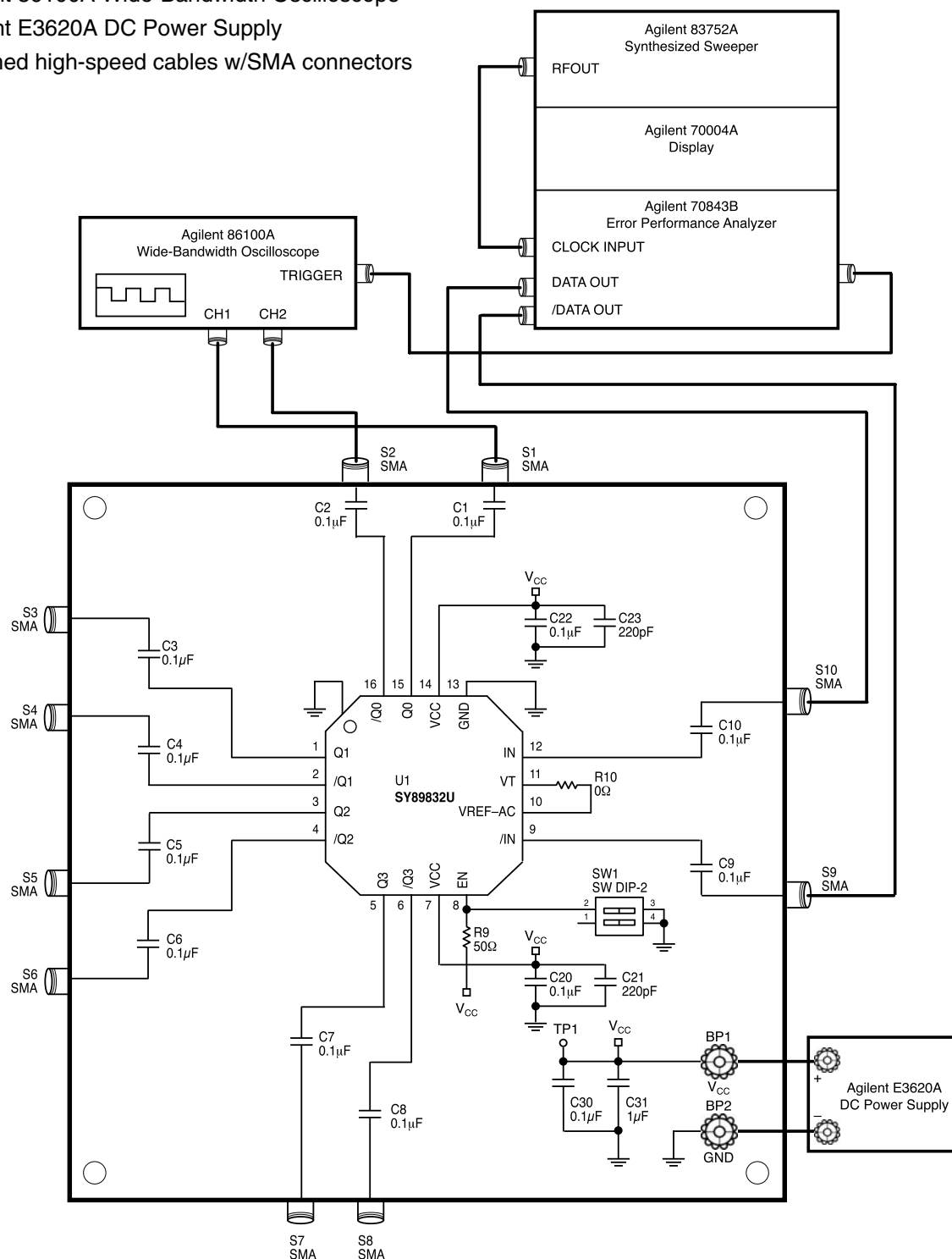
Figure 2. Setup for Measurements
