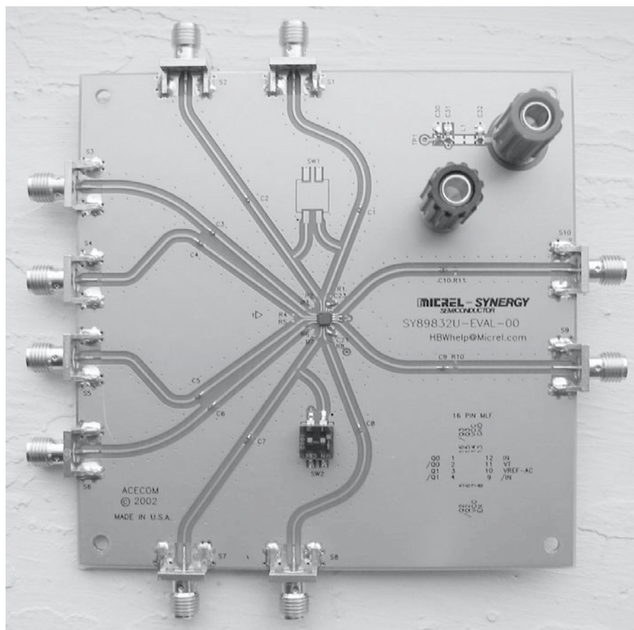
Figure 1. SY89832U Evaluation Board
