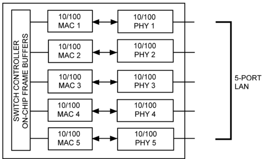
Figure 3. Standalone Switch
