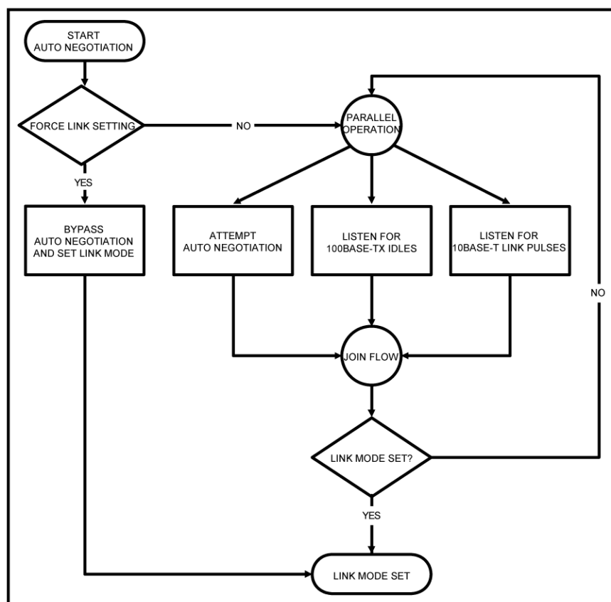
Figure 5. Auto Negotiation
