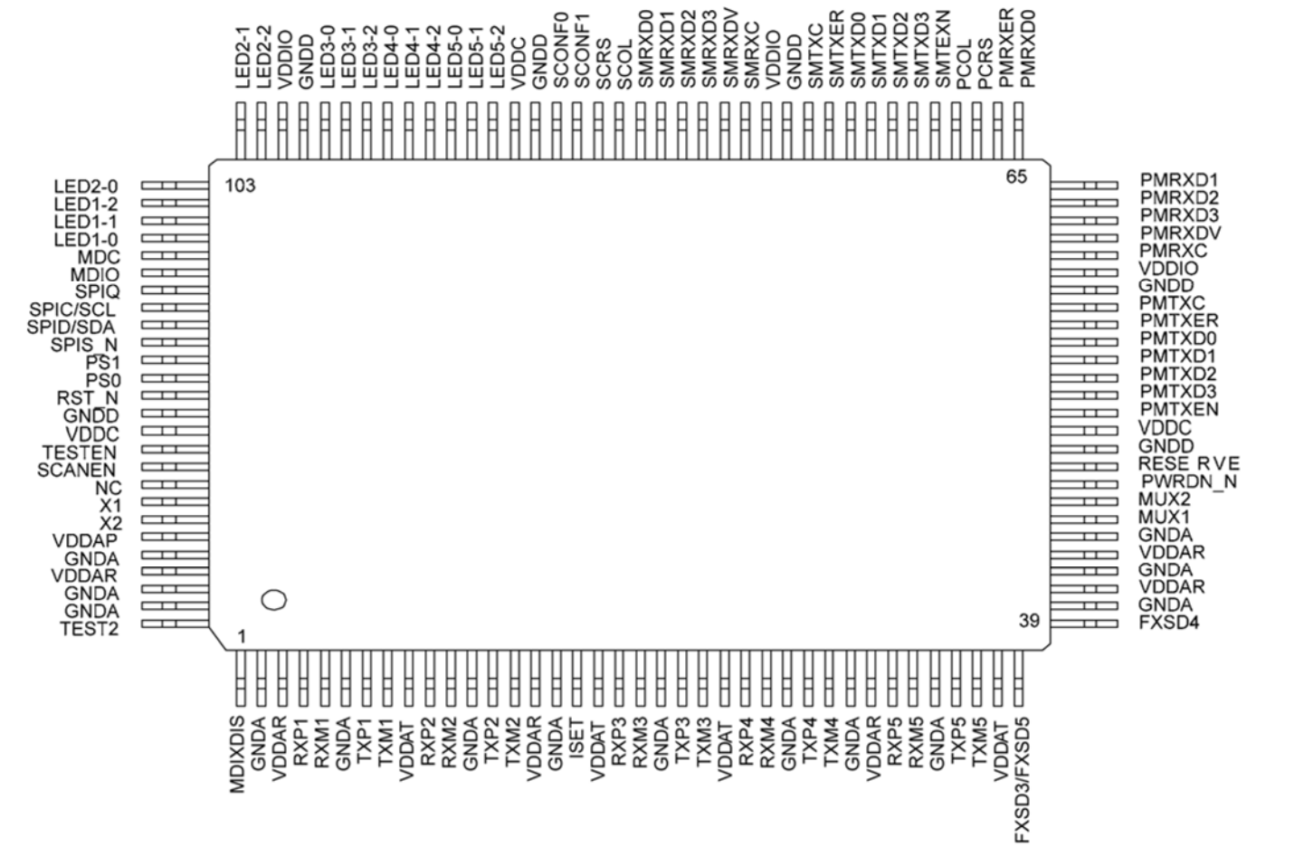
128-Pin PQFP
