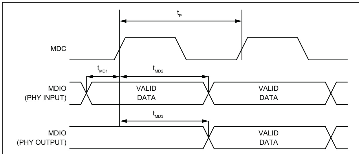
FIGURE 7-7: MDC/MDIO TIMING
