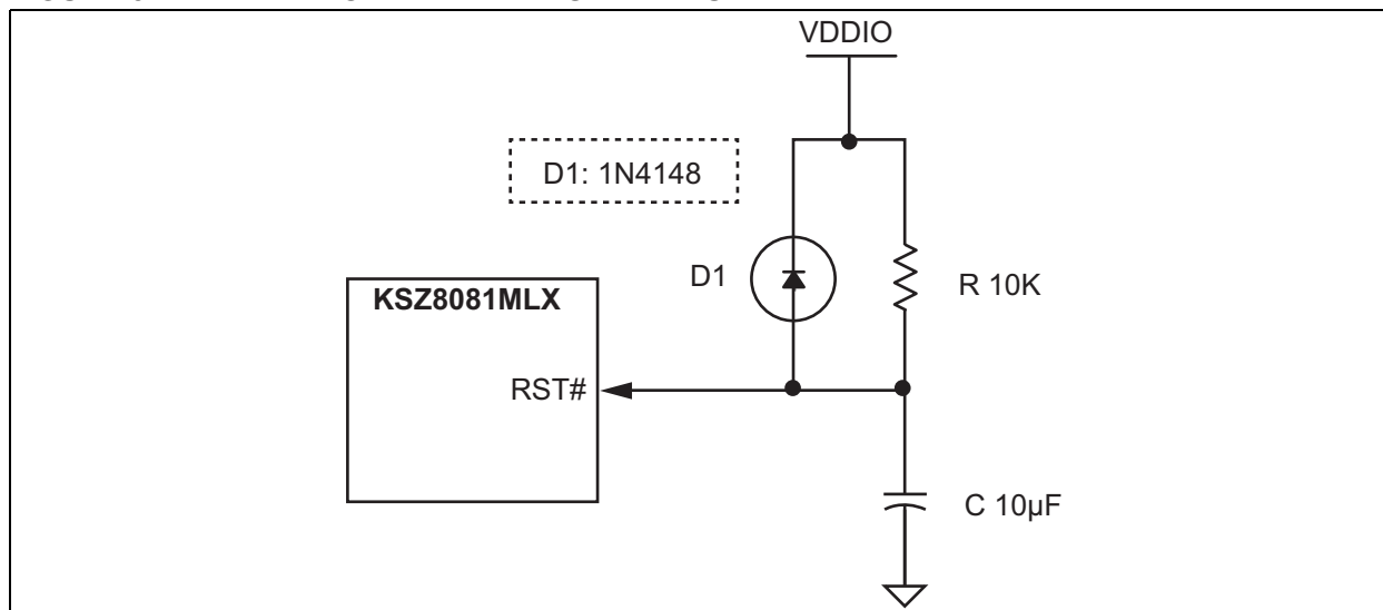
FIGURE 8-1: RECOMMENDED RESET CIRCUIT
