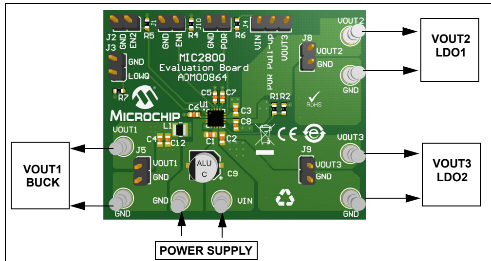
FIGURE 2-1: MIC2800 Evaluation Board – Test Points Description.
