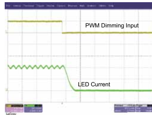
(c) PWM Dimming Fall Time Time Scale : 10μs/div
