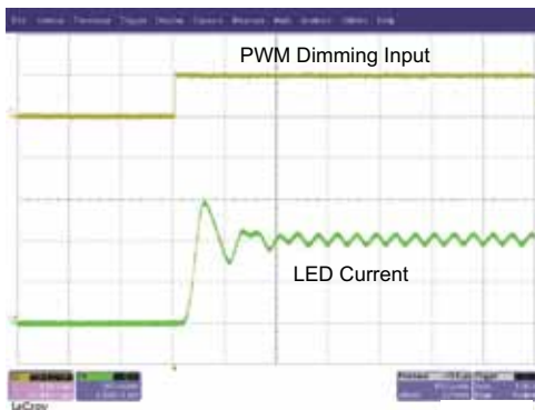
(b) PWM Dimming Rise Time Time Scale : 10μs/div
