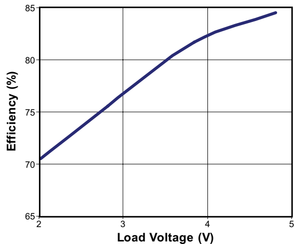
Fig. 3. Efficiency vs. Load Voltage Plot (@13.5V input)
