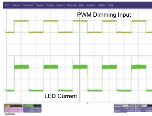
(a) PWM Dimming Performance Time Scale : 1ms/div
