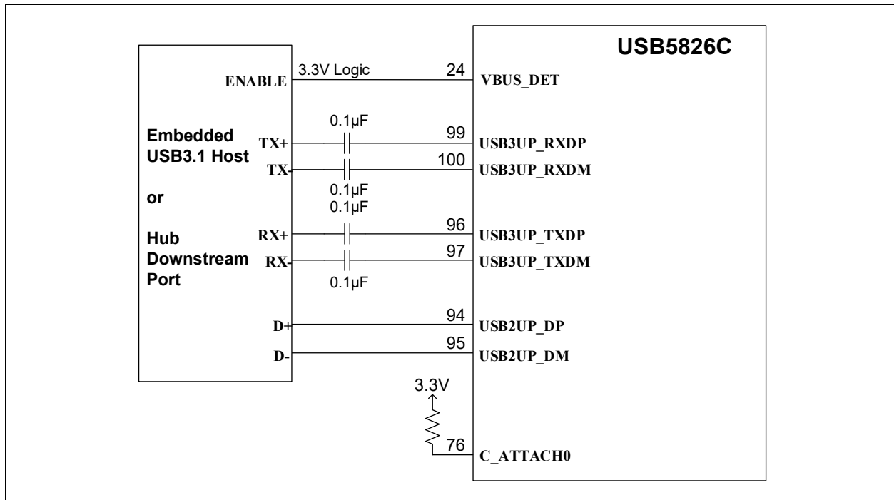
FIGURE 4-2: UPSTREAM PORT EMBEDDED HOST USB CONNECTIONS
