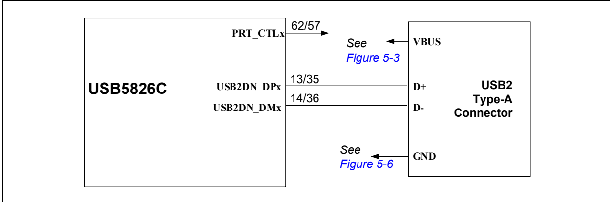
FIGURE 4-5: DOWNSTREAM PORT USB2.0-ONLY TYPE-A USB CONNECTIONS
