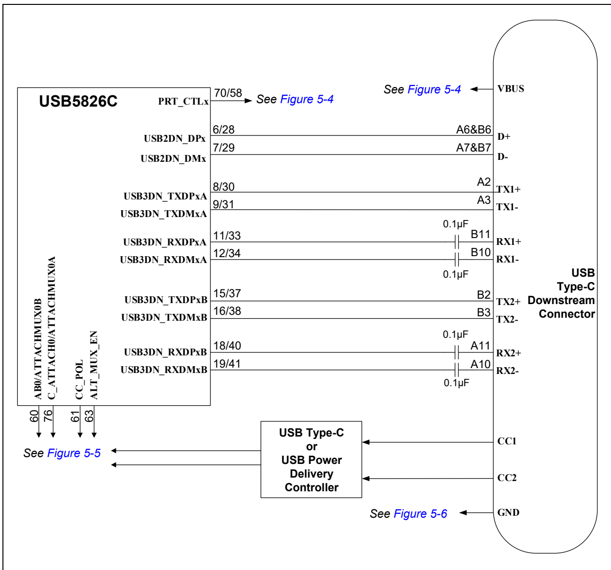
FIGURE 4-3: DOWNSTREAM PORT TYPE-C USB DATA CONNECTIONS
