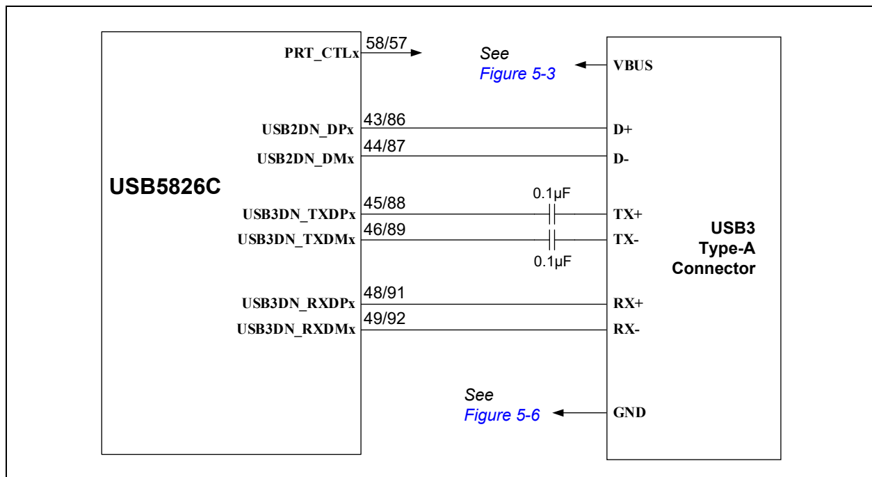
FIGURE 4-4: DOWNSTREAM PORT TYPE-A USB CONNECTIONS
