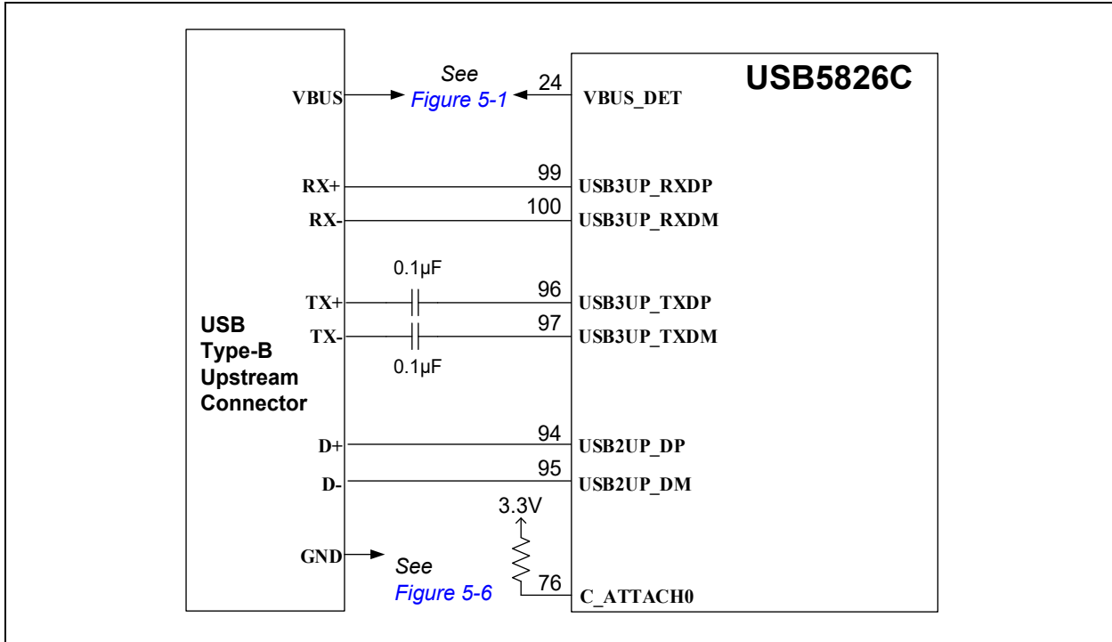
FIGURE 4-1: UPSTREAM PORT TYPE-B USB DATA CONNECTIONS
