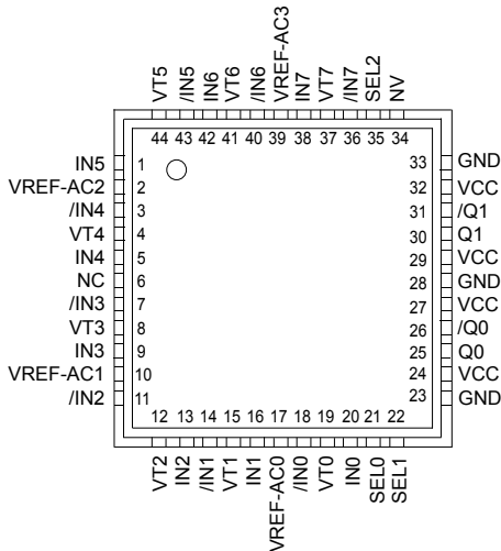
44-Pin QFN
