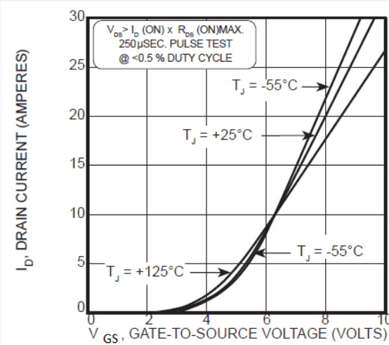
Figure 1-3. Transfer Characteristics
