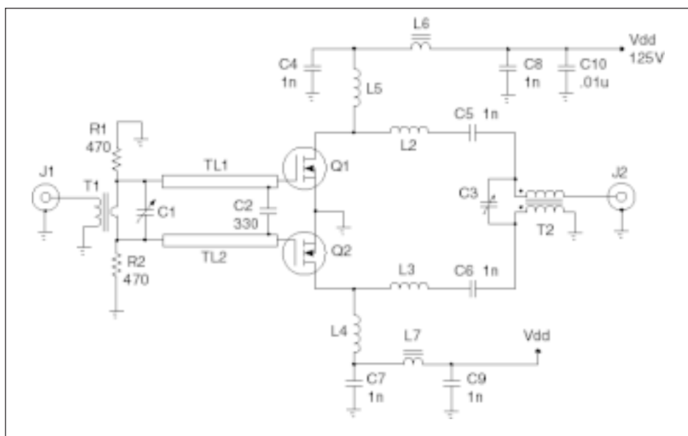
■ Figure 3. Amplifier circuit diagram.
