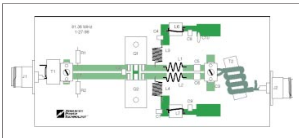
■ Figure 4. Parts placement pictorial diagram.
