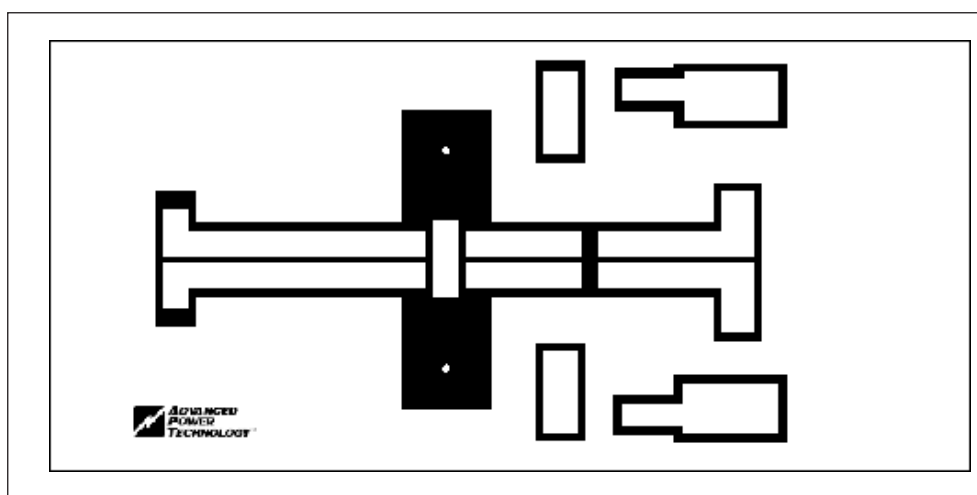
■ Figure 5. PWB photomaster. (Note: Not to scale)
