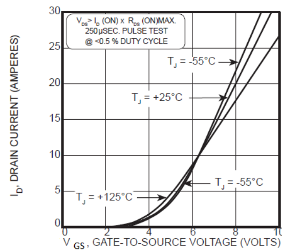
Figure 1-3. Transfer Characteristics
