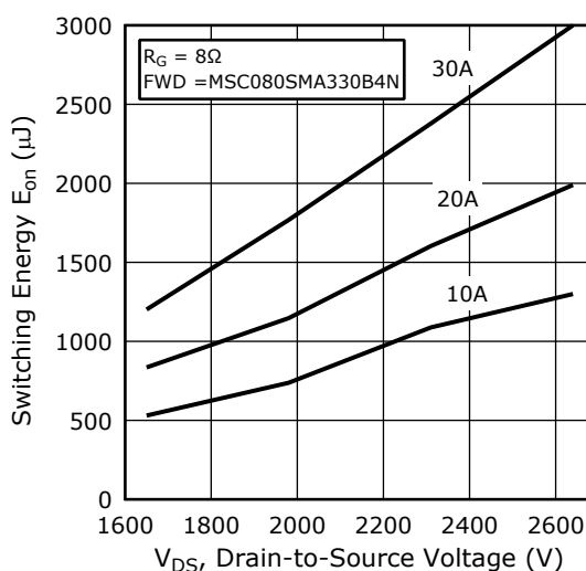
Figure 1-12. Switching Energy E_{on} vs. V_{DS} & I_D
