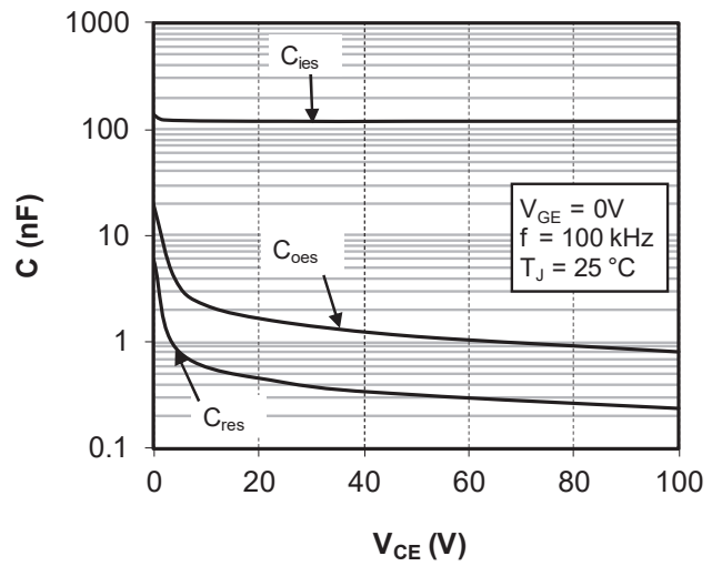
Figure 1-9. Capacity Characteristics
