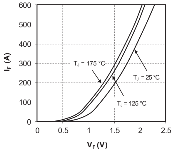
Figure 1-12. Forward Characteristics
