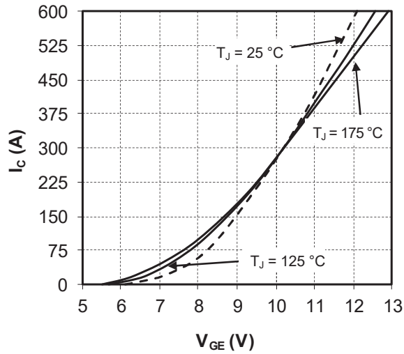
Figure 1-8. Transfer Characteristics
