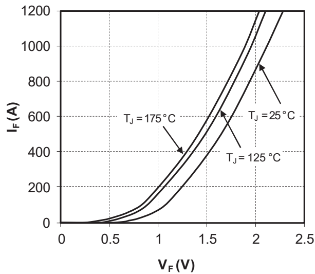
Figure 1-12. Forward Characteristics
