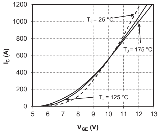
Figure 1-8. Transfer Characteristics
