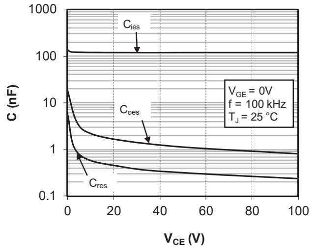
Figure 1-9. Capacity Characteristics
